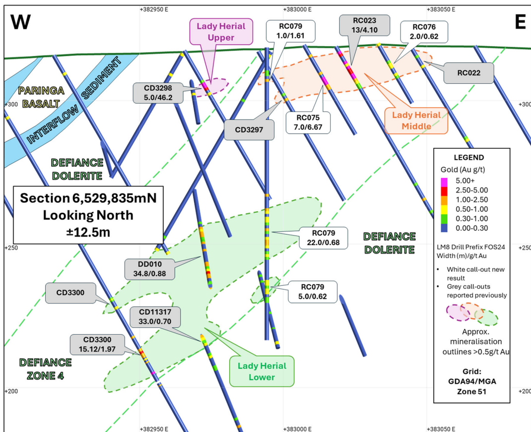
Figure 3: Cross section 6,529,835mN through the Middle and Lower Structure with location of new results.
