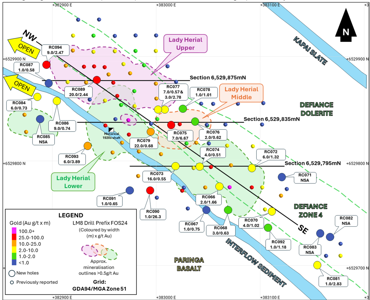
Figure 1: Plan view of the emerging Lady Herial mineralised gold system depicting Lower, Middle and Upper Structures plunging to the NW.
