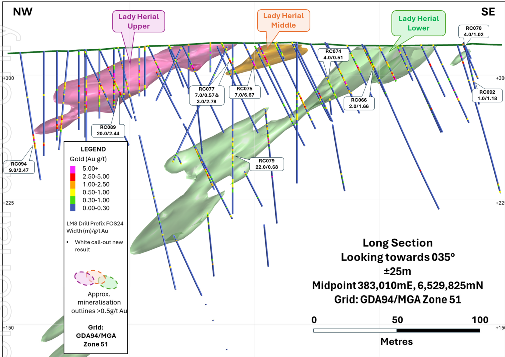
Figure 5: Long section NW-SE (+/- 25m clip) highlighting the stacked nature of Lower, Middle and Upper Structures over a vertical extent of between 75m and 150m.
