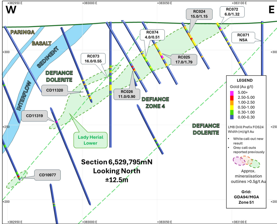
Figure 4: Cross section 6,529,795mN highlighting the Lower Structure at Lady Herial and new results.
