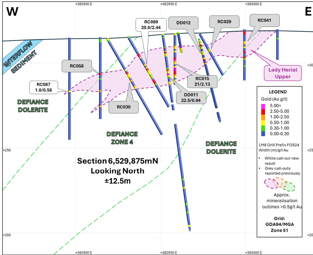
Figure 2: Cross section 6,529,875mN through the Upper Structure illustrating location of new results.
