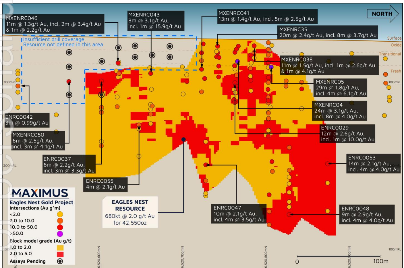
Figure 1 – Eagles Nest Gold Deposit long-section displaying Mineral Resource Estimate (MRE) block model and drill hole pierce points, including black points indicating assays pending.
