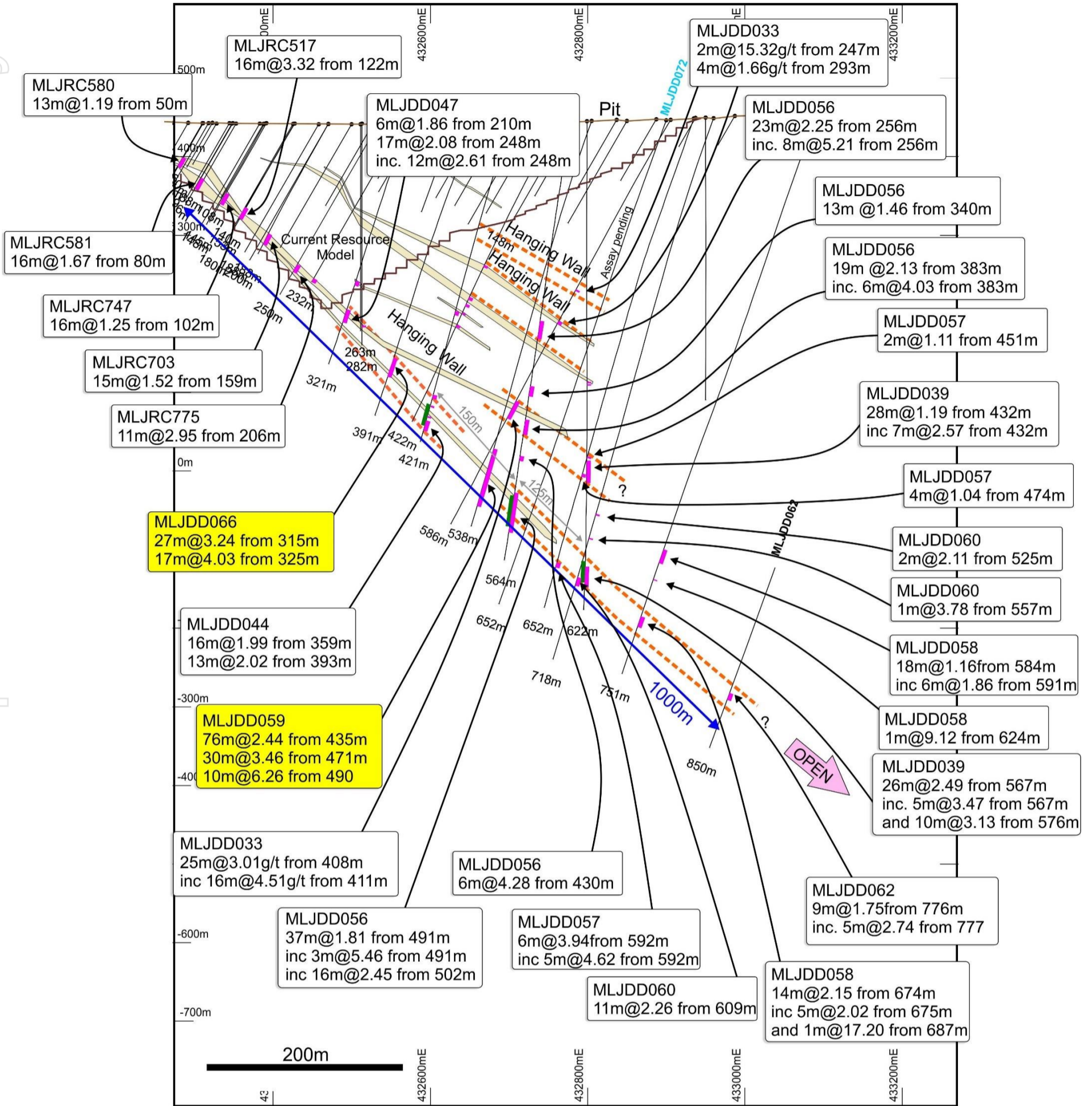
Figure 2. Composite section for LJN4 central area showing high-grade dipping gold zone containing resource model outline, proposed open pit and MLJDD039, 44, 47, 56, 57, 58, 59, 60, 62, 66 being part of a very large 1000m down dip mineralised main zone.
