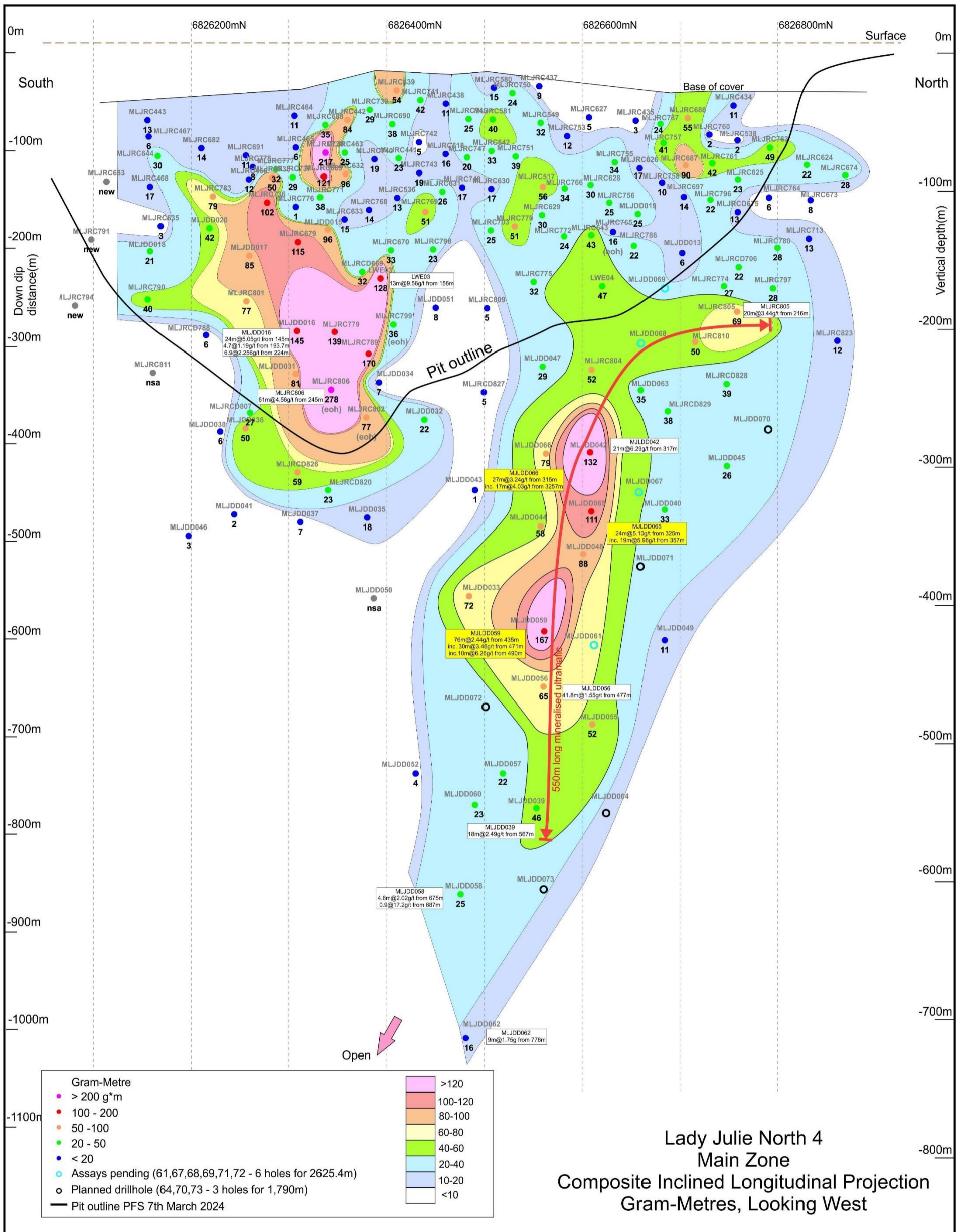
Figure 1. Composite Inclined Longitudinal Projection of LJV4 in gram-metres. Highlighting continuous mineralisation over the whole 750m strike length, being open at depth in the northern altered ultramafic zone and showing a 550m long SE plunging core zone. New drilled holes awaiting assays (in blue) and further planned holes (in black). New drill results in yellow label and older results in white.
