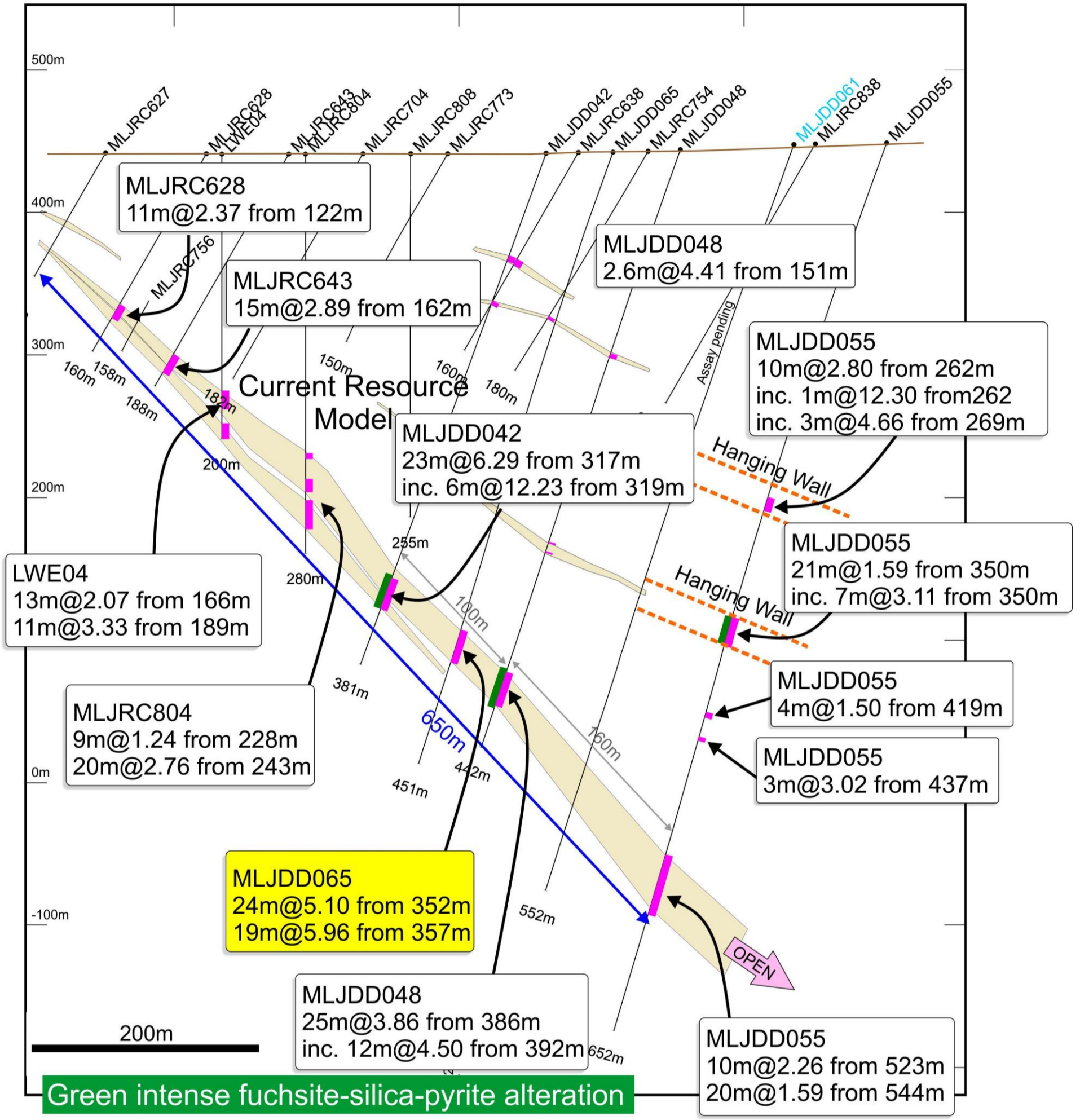
Figure 3. Cross section for LNJ4 northern area showing high-grade dipping gold zone containing resource model outline and MLJDD042, 48, 55, 65 being part of a large 650m down dip footwall down dip extension of 160m from MLJDD048. MLJDD061 is waiting for assay and being planned to be drilled respectively.
