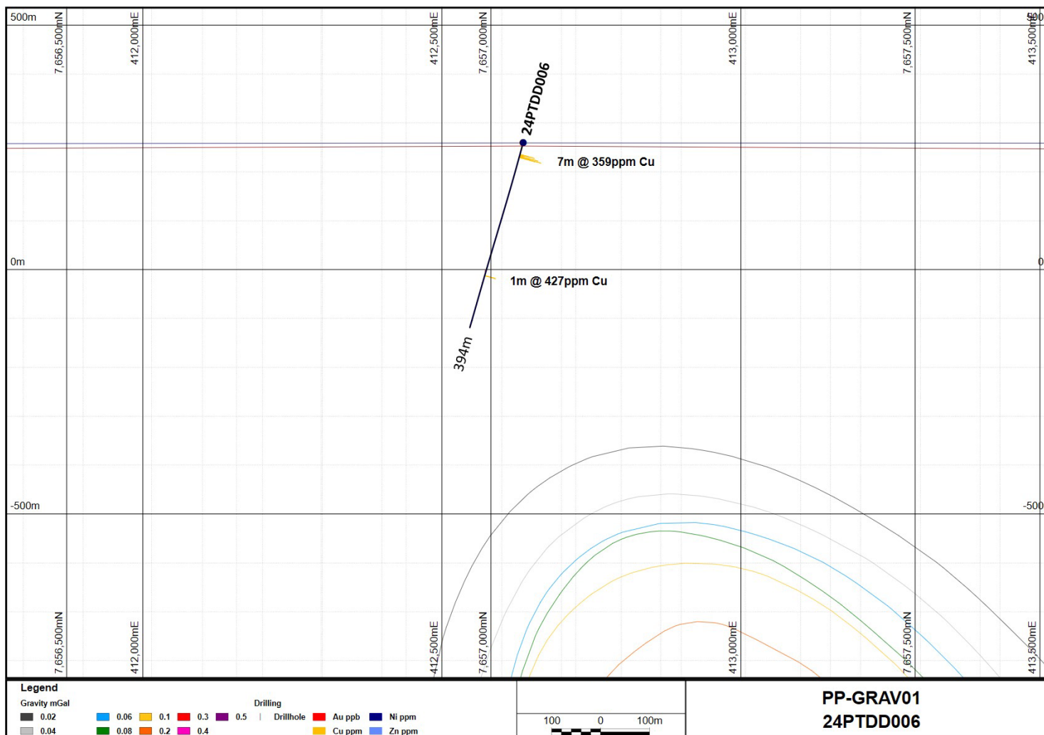
Figure 15: PP-GRAV01 cross-section for 24PTDD006 (refer to Figures 3, 4 and 8) showing drill intercepts and ground gravity isosurfaces. NB: 500m elevation (RL) and north-south grid, looking toward 325° GDA2020 / MGA Zone 51 Grid.
