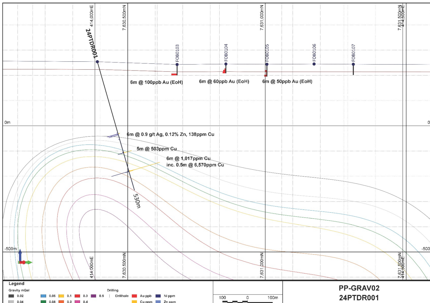
Figure 11: PP-GRAV02 cross-section for 24PTDR001 (refer to Figures 3 to 6) showing drill intercepts and ground gravity isosurfaces. NB: 500m elevation (RL) and north-south grid, looking toward 315° GDA2020 / MGA Zone 51 Grid.
