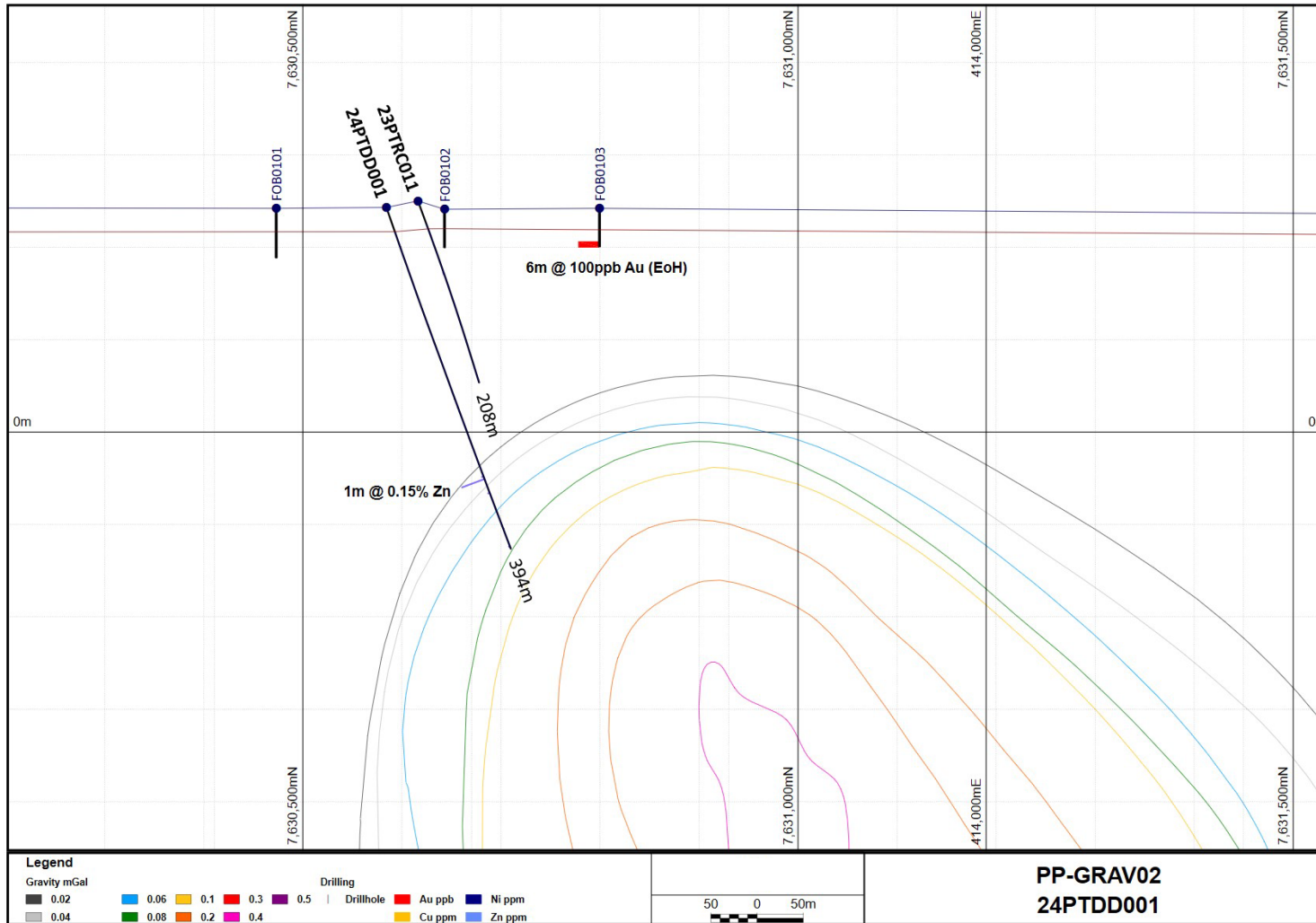
Figure 12: PP-GRAV02 cross-section for 24PTDD001 (refer to Figures 3 to 6) showing drill intercepts and ground gravity isosurfaces. NB: 500m elevation (RL) and north-south grid, looking toward 295° GDA2020 / MGA Zone 51 Grid.
