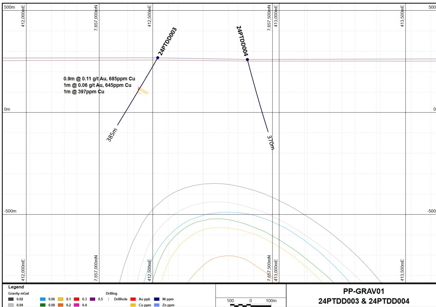
Figure 14: PP-GRAV01 cross-section for 24PTDD003 and 24PTDD004 (refer to Figures 3, 4 and 8) showing drill intercepts and ground gravity isosurfaces. NB: 500m elevation (RL) and north-south grid, looking toward 325° GDA2020 / MGA Zone 51 Grid.
