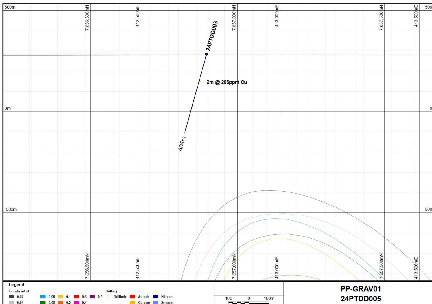
Figure 16: PP-GRAV01 cross-section for 24PTDD005 (refer to Figures 3, 4 and 8) showing drill intercepts and ground gravity isosurfaces. NB: 500m elevation (RL) and north-south grid, looking toward 325° GDA2020 / MGA Zone 51 Grid.
