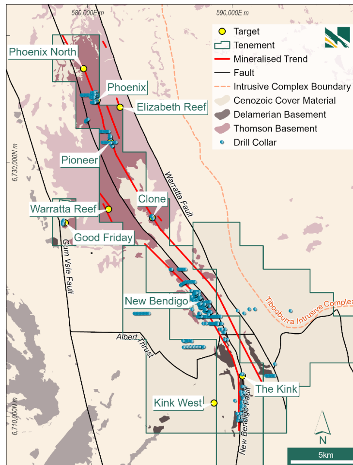
Figure 9: Tibooburra project tenure, with geology, drill collars, main prospects, highlighting multiple parallel mineralised trends.
