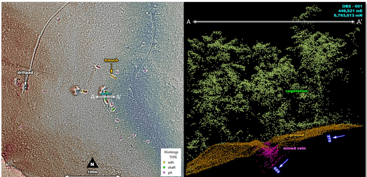
Figure 5: OBS-001: Plan view showing trenches, shaft and adit and cross section showing mined vein dipping 55^{\circ} to 270^{\circ} TN. The vein has multiple shafts sunk, with an adit 40m to the WNW trending 102^{\circ} TN towards the vein. A drill pad is also located 140m to the WNW.
