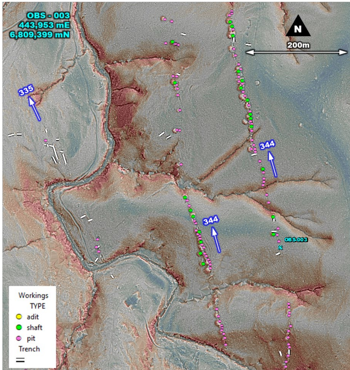
Figure 4: OBS-003 – Plan view showing two parallel, 344 o TN trending veins heavily worked over >750m of strike. A third vein is more subtly defined by pits and trenches located 360m to the West, trending 335 o TN.
