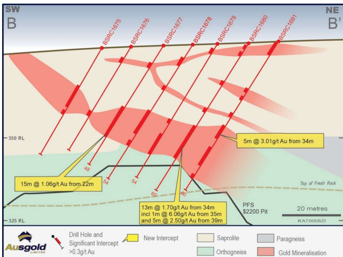
Figure 4 – Cross-section B-B' across the southern-most line of the Grade Control program
