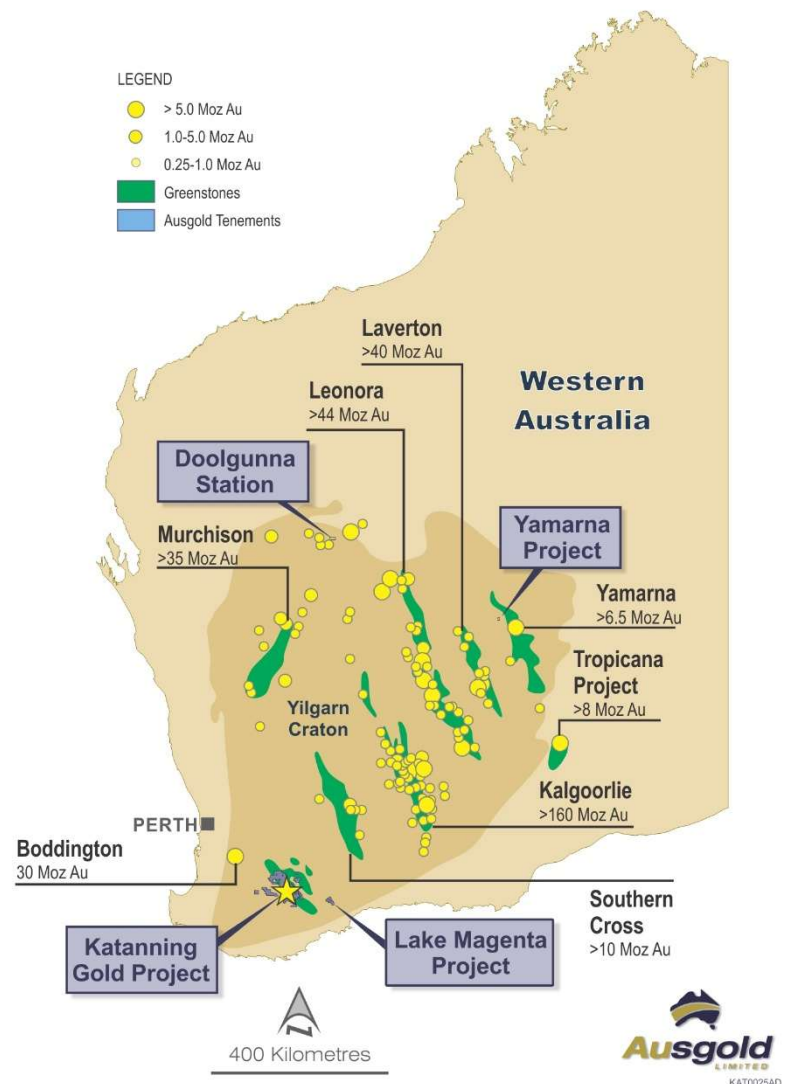
Figure 6 - Statewide map showing the KGP, other Ausgold projects and mineralised greenstone belts
