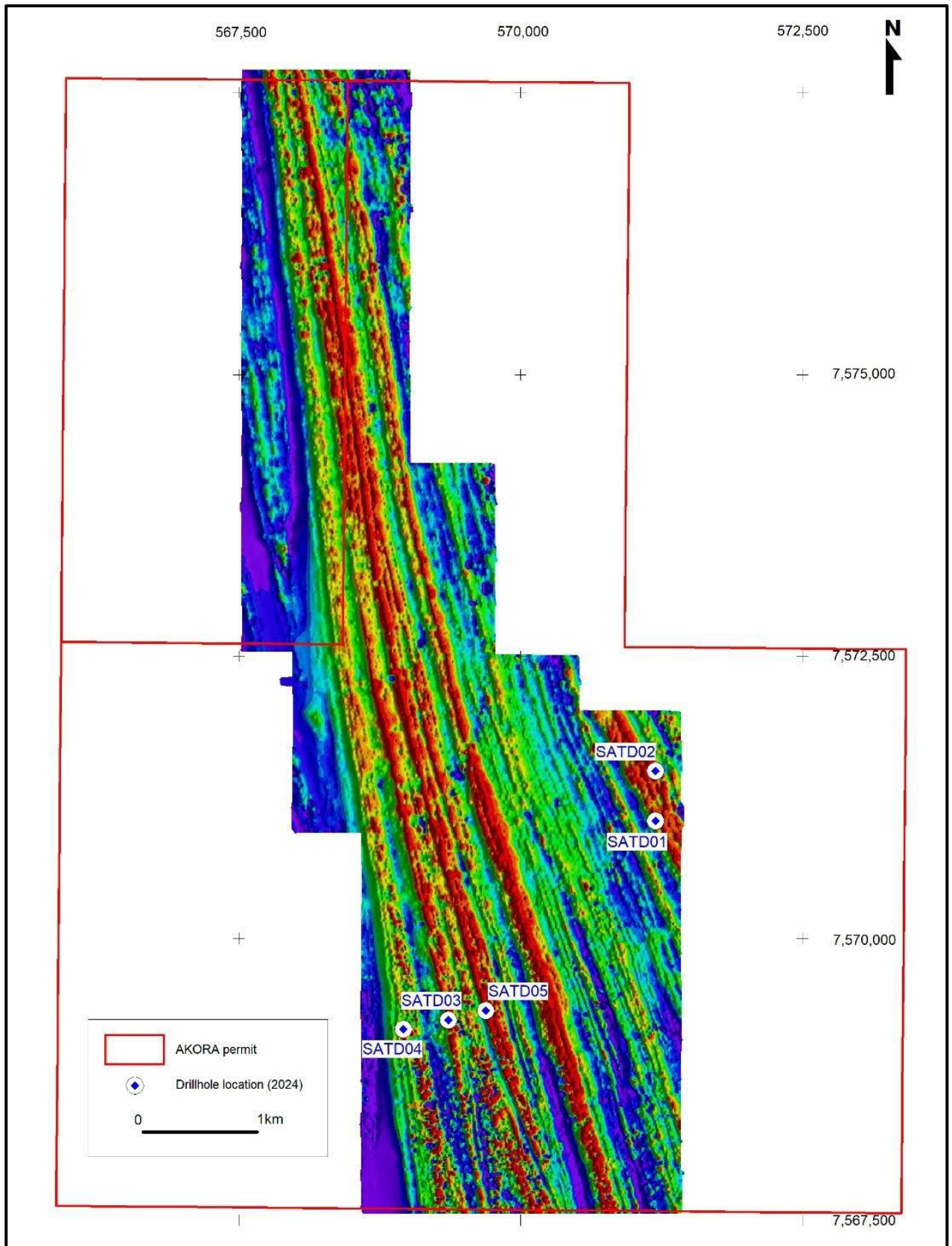
Figure 1: Map showing magnetic anomalies and drillhole locations at Satrokala.
