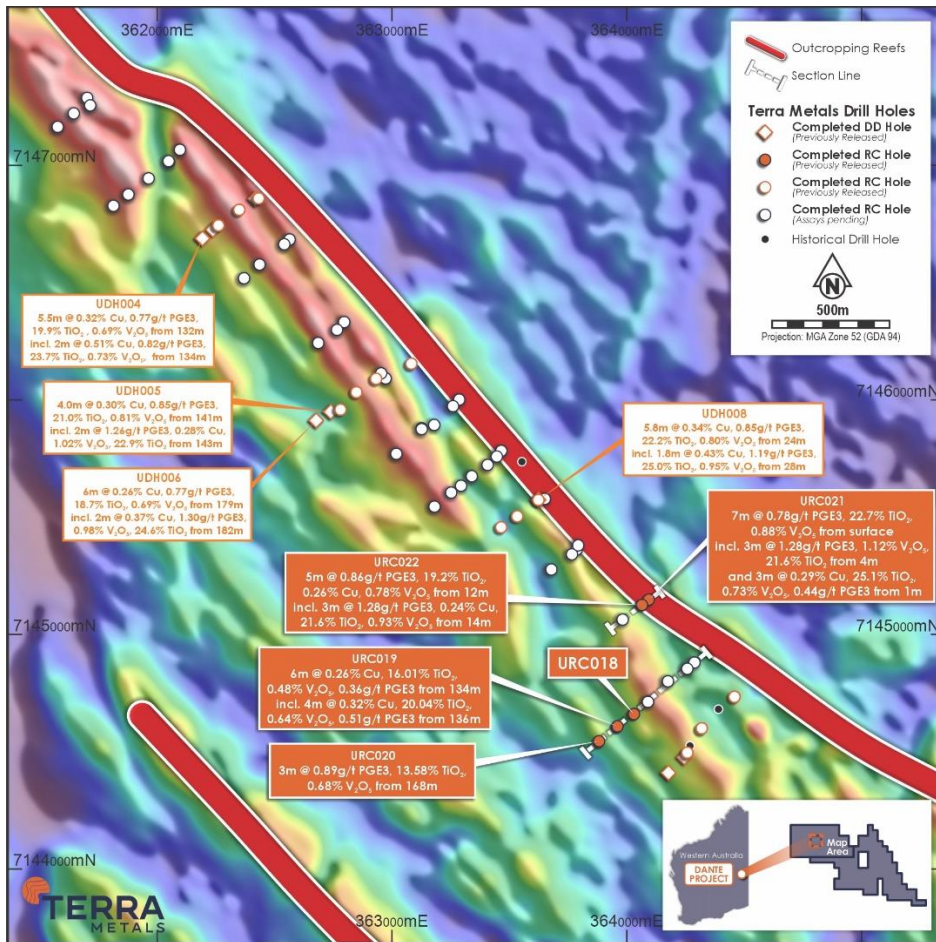
Figure 3. Reef 1 North inset, showing recent drilling over TMI magnetics.
