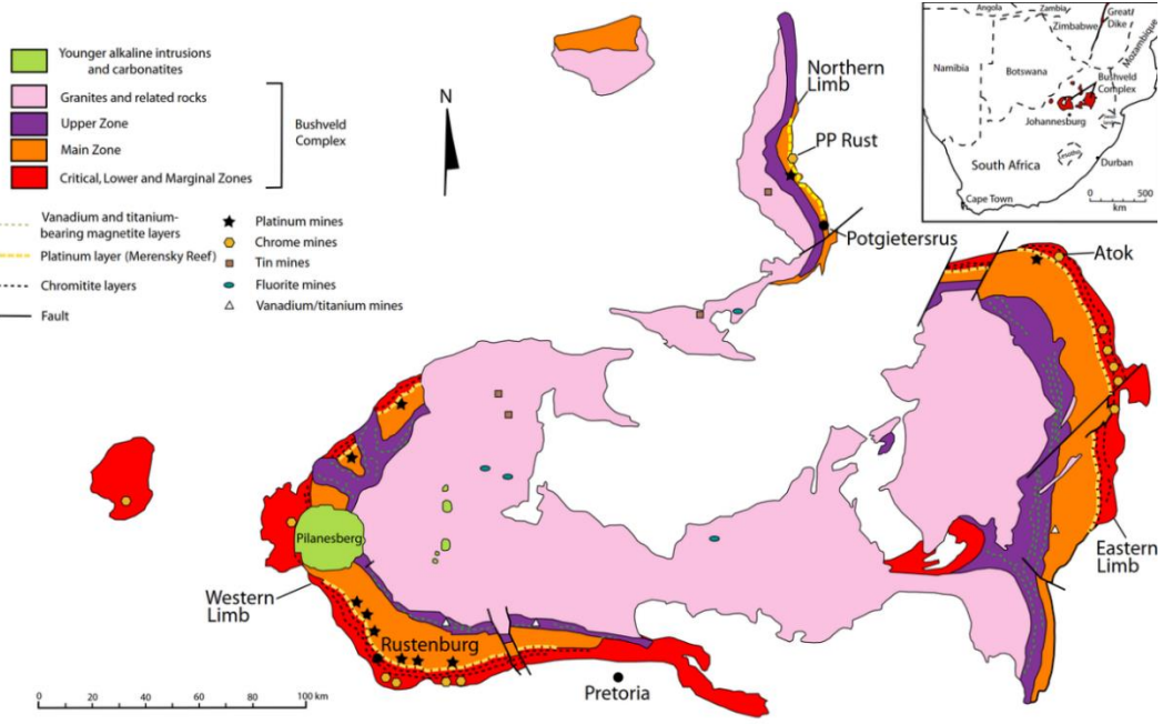
Figure 6. Schematic of the Bushveld Complex, South Africa, showing the various metallogenic provinces within the complex which includes specific layers which are commercial enriched in PGEs, Copper, Nickel, Titanium, Vanadium, and Chromium (source: USGS Open-File Report 2005-1294-E).
