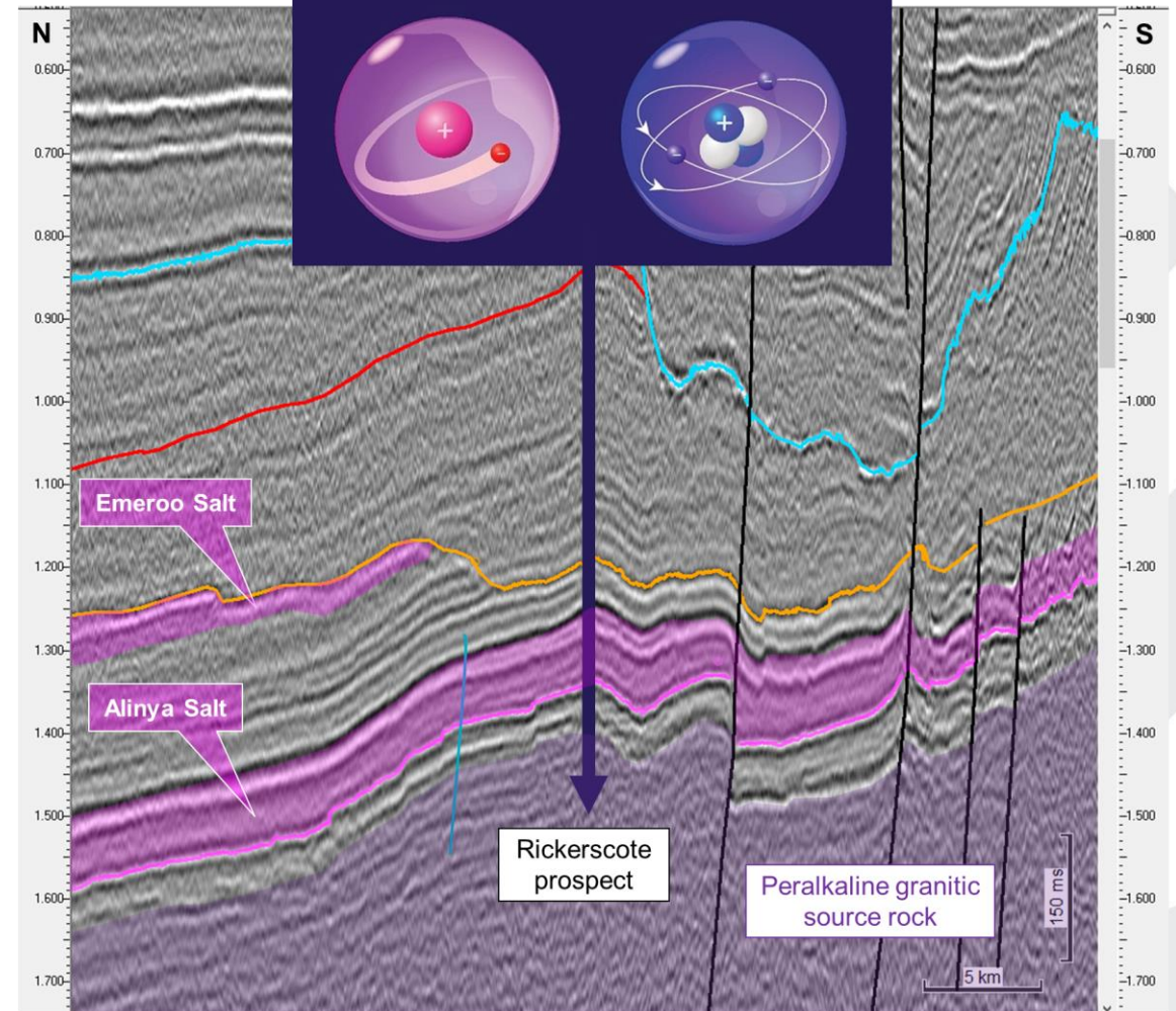
2D Seismic Line over Rickerscote Prospect
