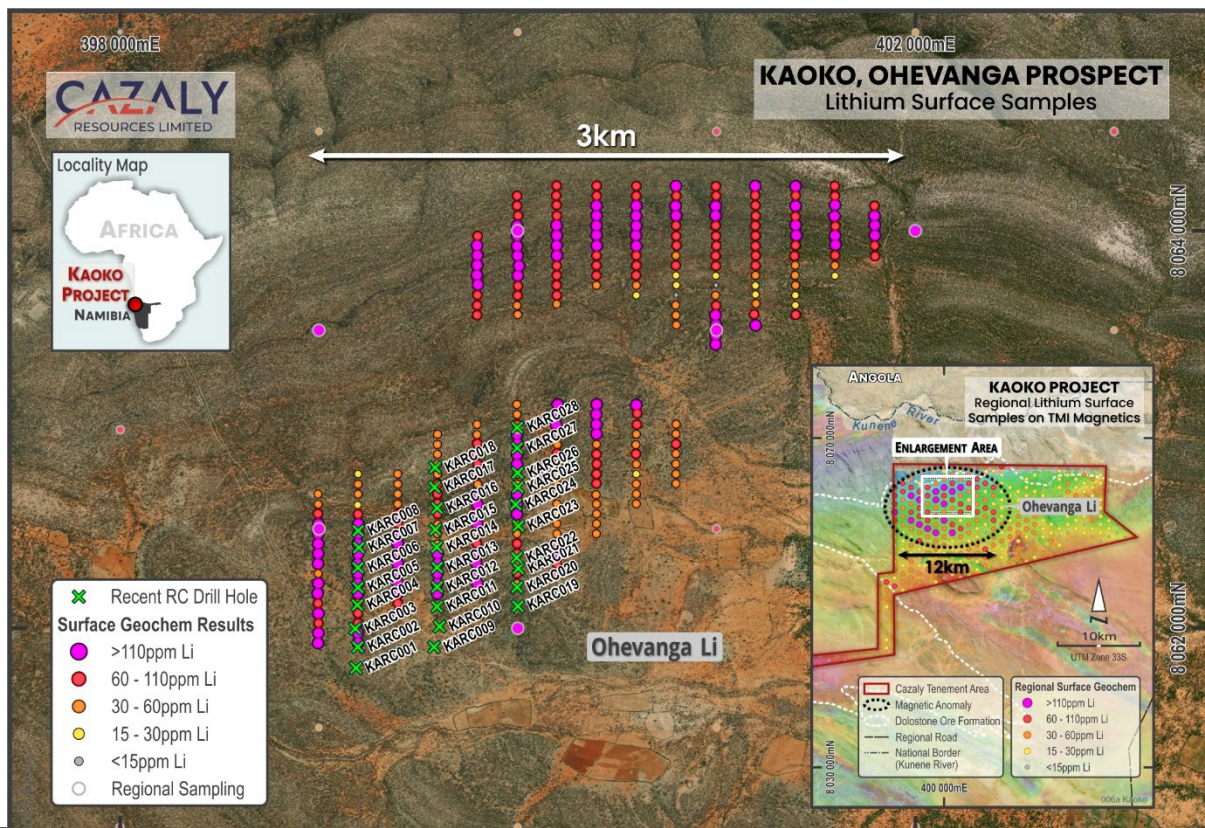
Figure 1. Location of the Ohevanga lithium anomaly and RC drill collars.
