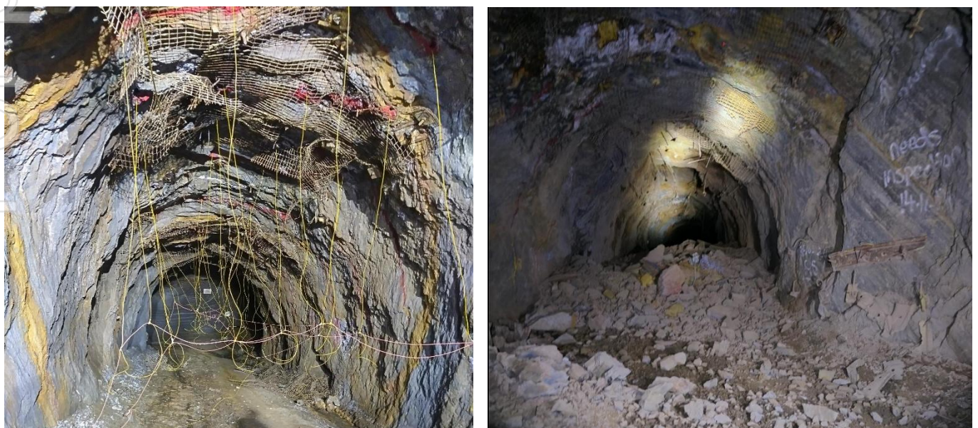
Figure 4. Level 1: Charged (LHS) & blasted (RHS) to establish ventilation to Upper North Lode (UNL).
