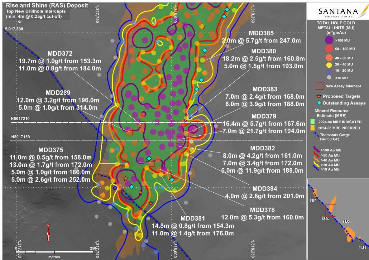
Figure 1. Plan of RAS metal unit (or gram.metre) map with pierce points of new drilling.
