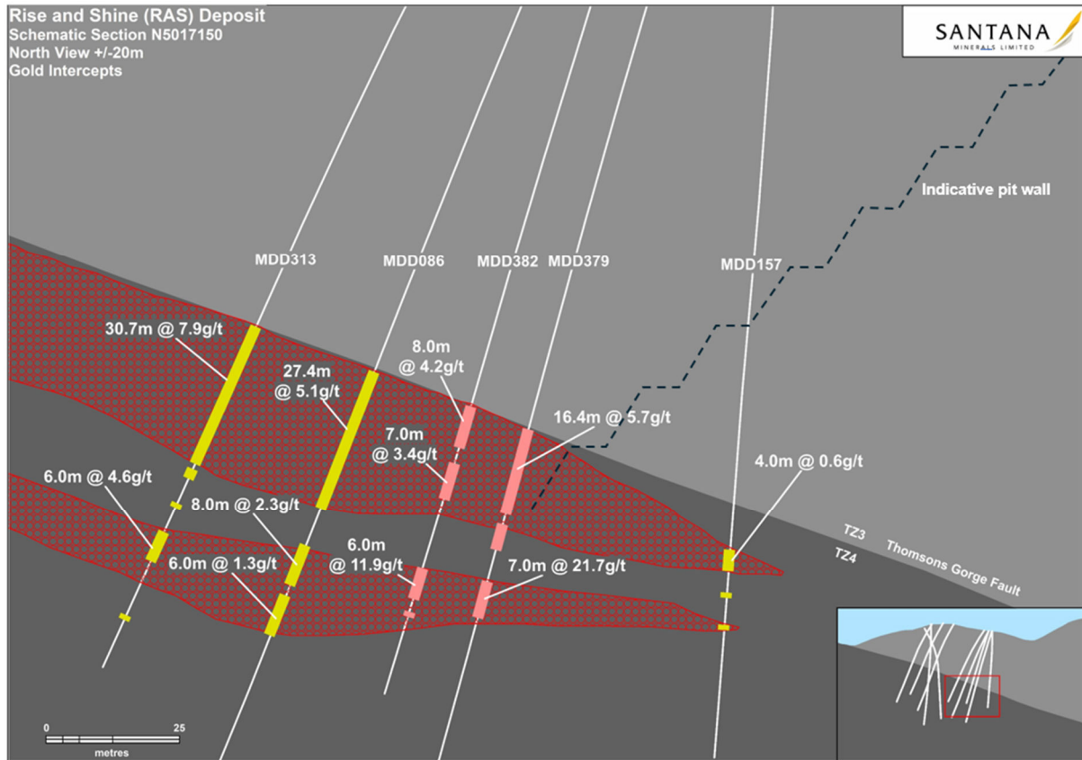
Figure 2. N5017150 section showing new intersections of MDD379 and MDD382 (in pink).
