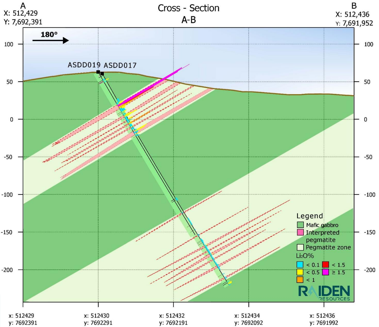
Figure 3: Cross section A-B
