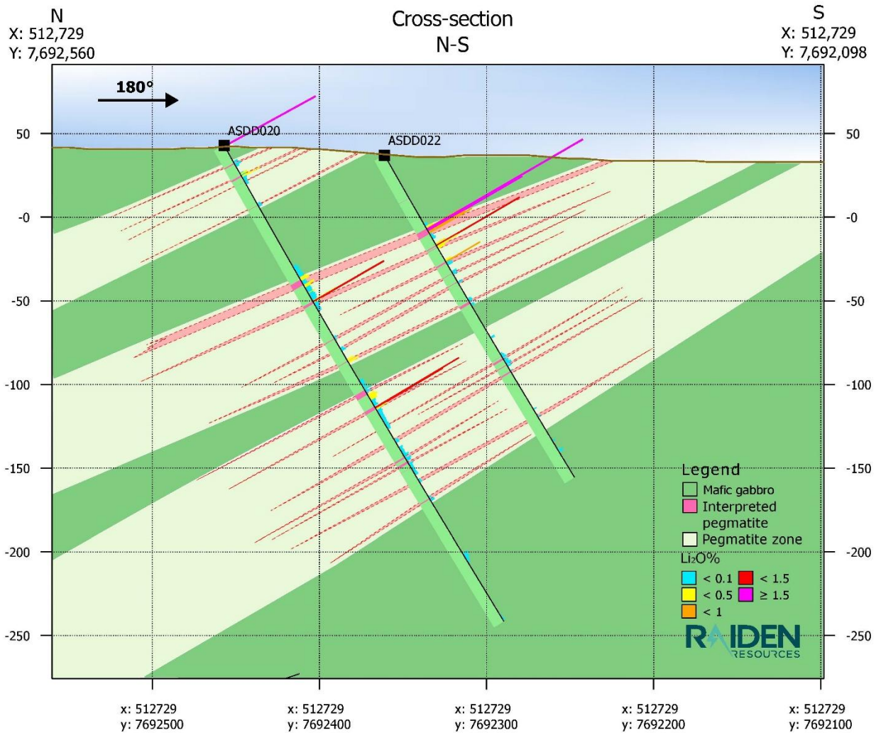
Figure 4: Cross section N-S
