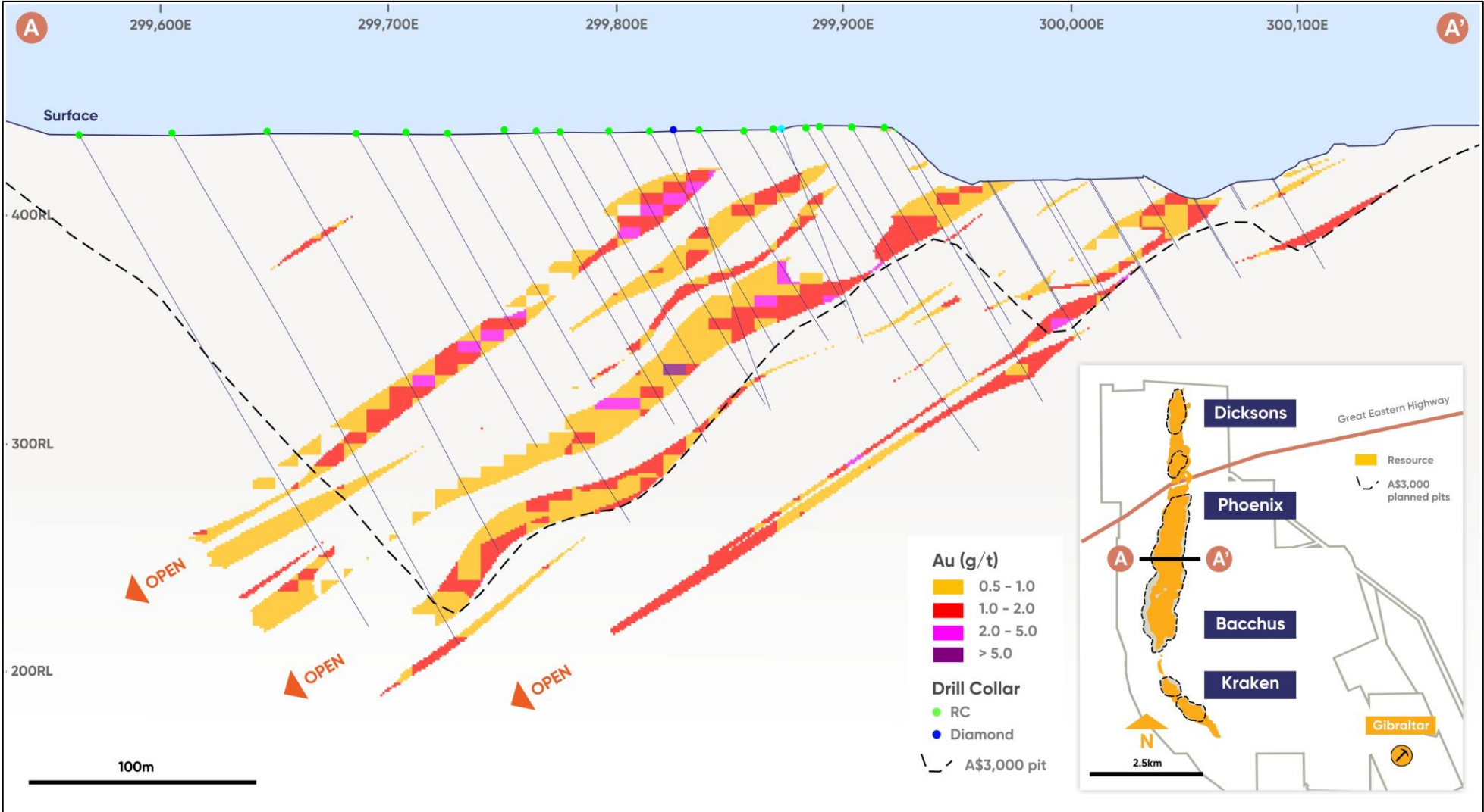
Bullabulling resource plan view and cross section showing gold grades, drilling intercepts and pit shells
