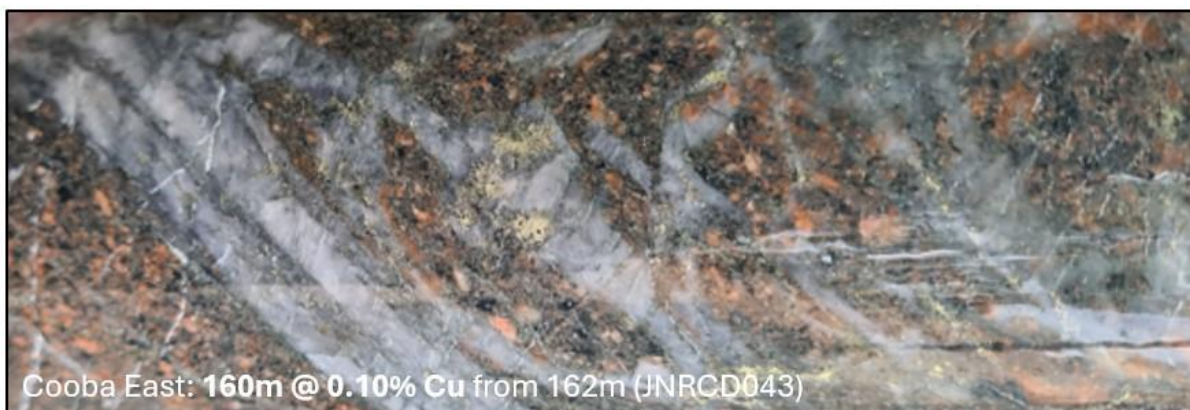
Photo 5. Example of quartz-pyrite-molybdenite-chalcopryrite porphyry veining developed in potassic altered monzonite from JNRCD043 at Cooba East associated with broad intersection of 160m @ 0.10% Cu from 162m.
