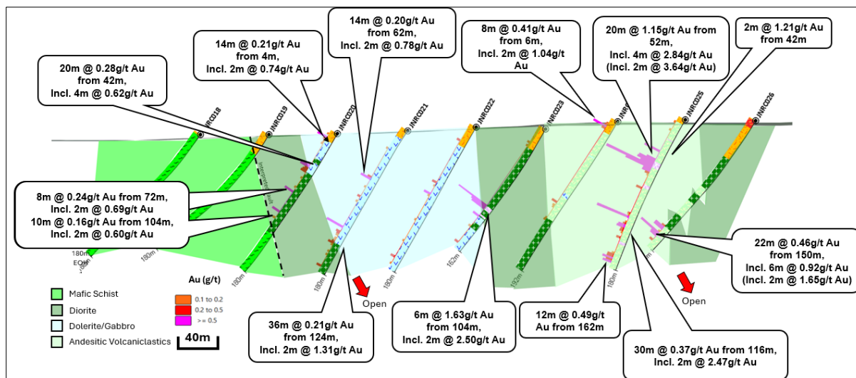
Figure 5. Section 6,145,250mN through Allawah from Figure 4 displaying salient gold intersections and interpreted geology. Note view looking north. 31
