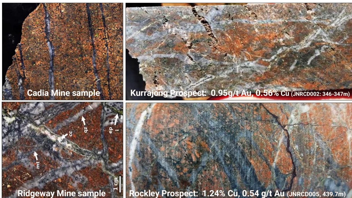
Photo 1. Cadia and Ridgeway Mine samples compared to Junee Project samples (Kurrajong and Rockley Prospects). Similar rock-types alteration, veining and Cu-Au mineralisation are observed which is considered highly encouraging.
