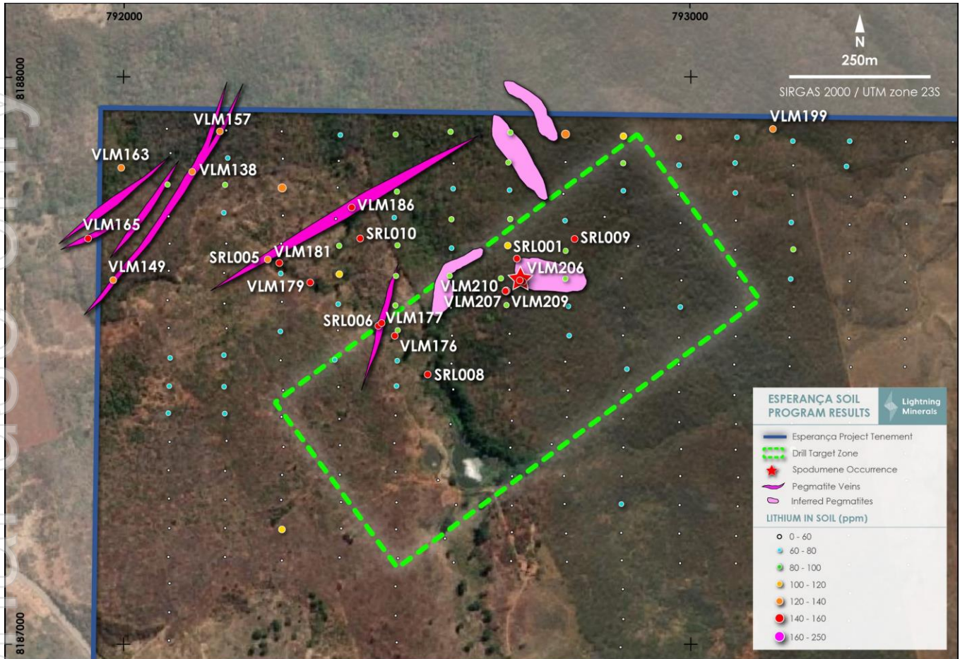
Figure 4: Soil sampling and rock chip sampling locations (lithium) at the Esperança project
