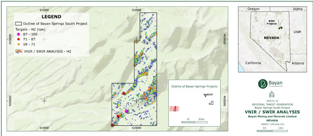
Figure 8: Bayan Springs South - targets defined based H 2 spectral endmember
