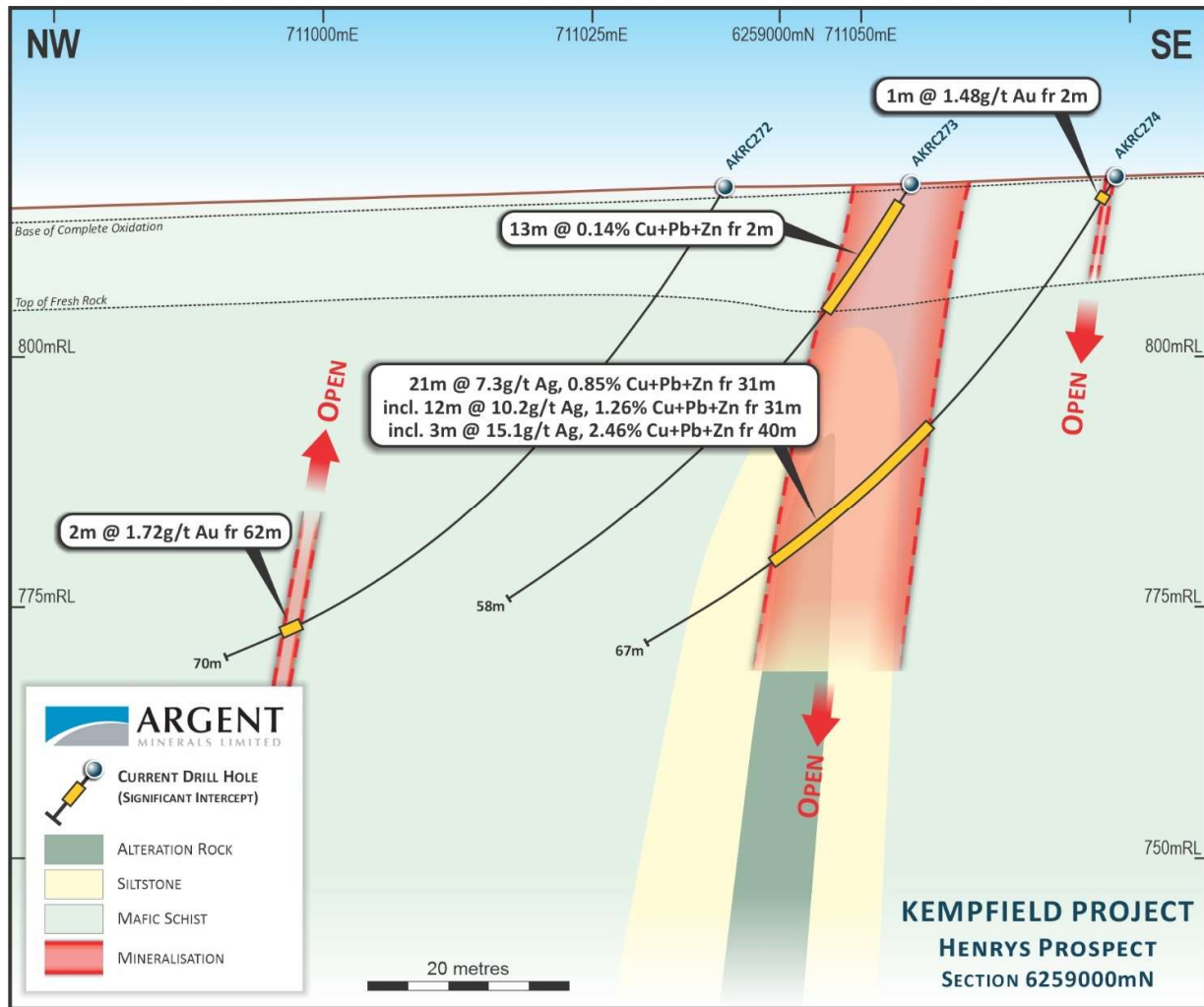
Figure 2 – Henry's Cross Section 6259000N highlighting mineralised intervals
