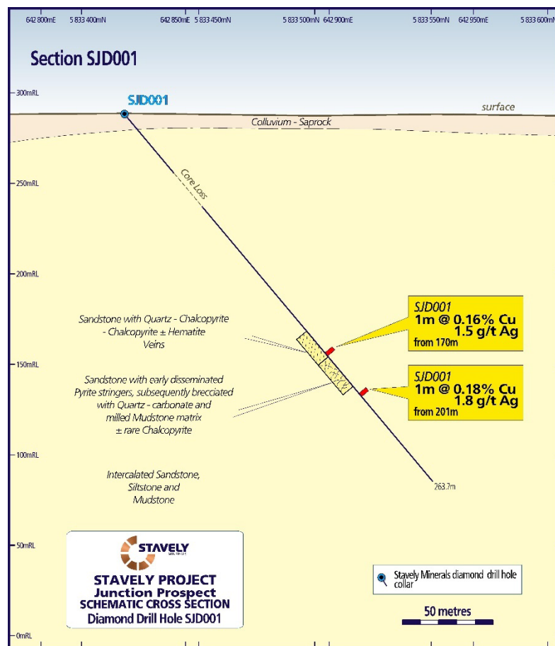
Figure 8. SJD001 drill section.
