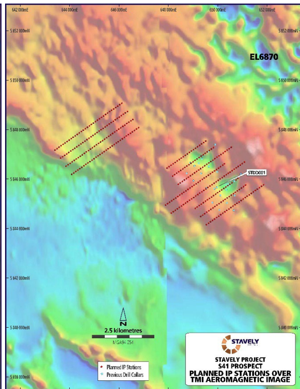
Figure 4. S41 gold prospect magnetic image with planned IP stations. The target demonstrates magnetic lows within a regional high – interpreted to reflect hydrothermal destruction of magnetite in the host andesite lavas.
