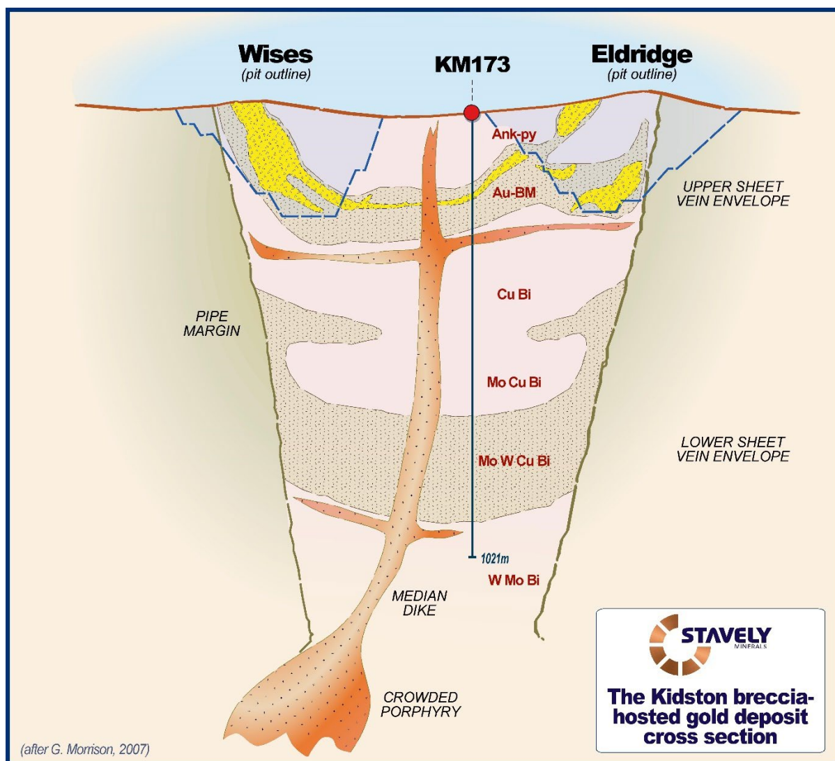
Figure 6. Cross-section of the Kidston breccia-hosted gold deposit showing the distribution of gold mineralisation (yellow) associated with a vertical metals zonation. Note that gold mineralisation is spatially restricted and associated with specific phases of brecciation and mineralisation. (Au-BM = gold and base metals, Ank-py = ankerite and pyrite) (After G. Morrison, 2007).
