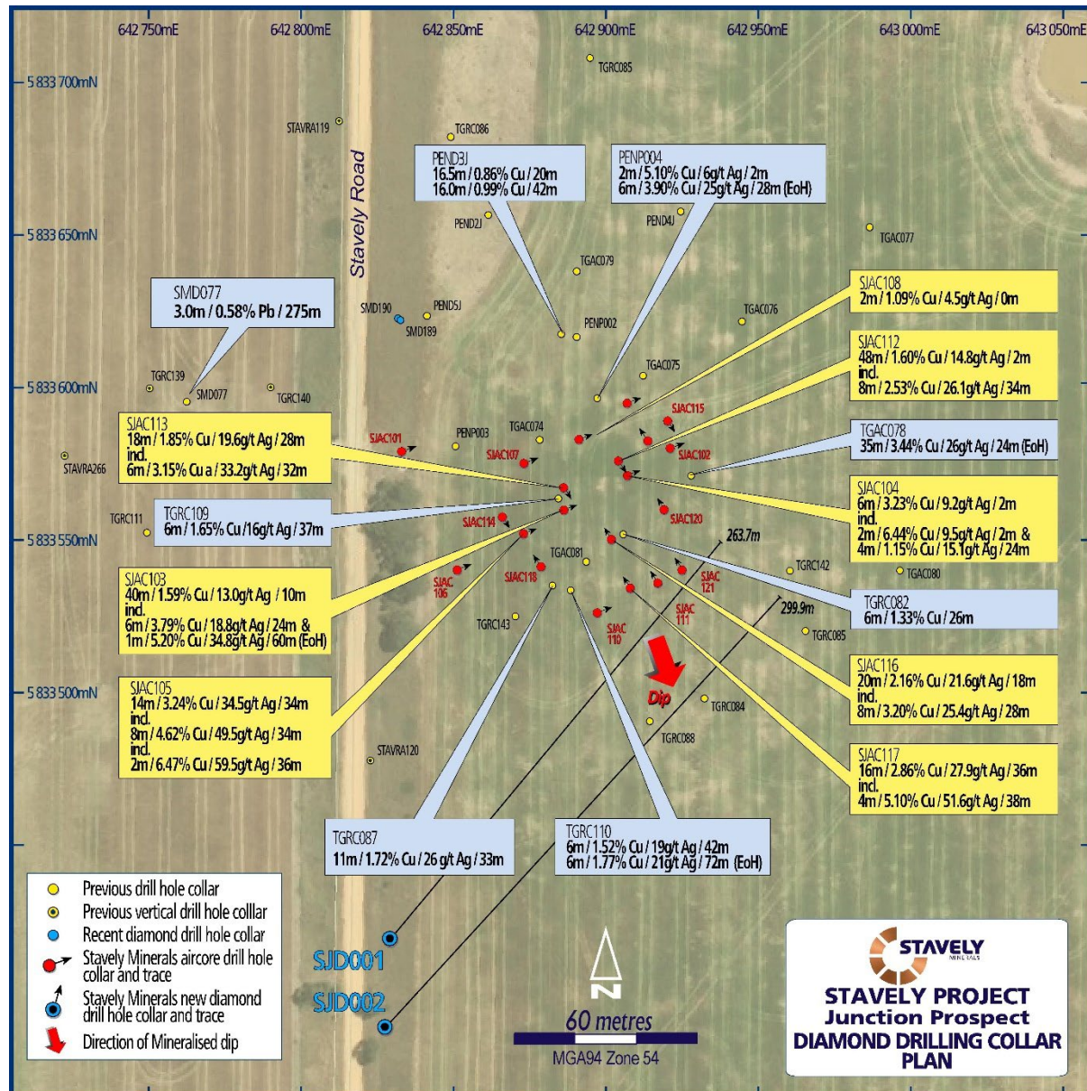
Figure 7. Junction Prospect drill collar plan with selected air-core/RC drilling intercepts. Light blue are historic intercepts from previous explorers, the yellow annotations are from recent air-core drilling, and the blue markers are the recent diamond drill collars.
