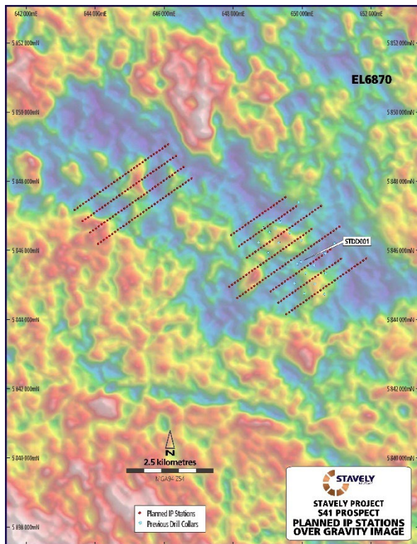
Figure 3. S41 gold prospect gravity image with planned IP stations. The target demonstrates gravity highs within a regional low.
