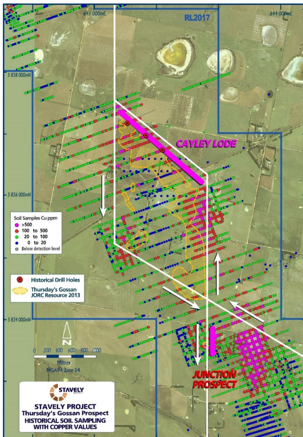
Figure 9. Cayley Lode and Junction Prospect location map with soil copper geochemistry (coloured dots) and structural context. Note the very large copper-in-soils geochemical anomaly east of Junction.
