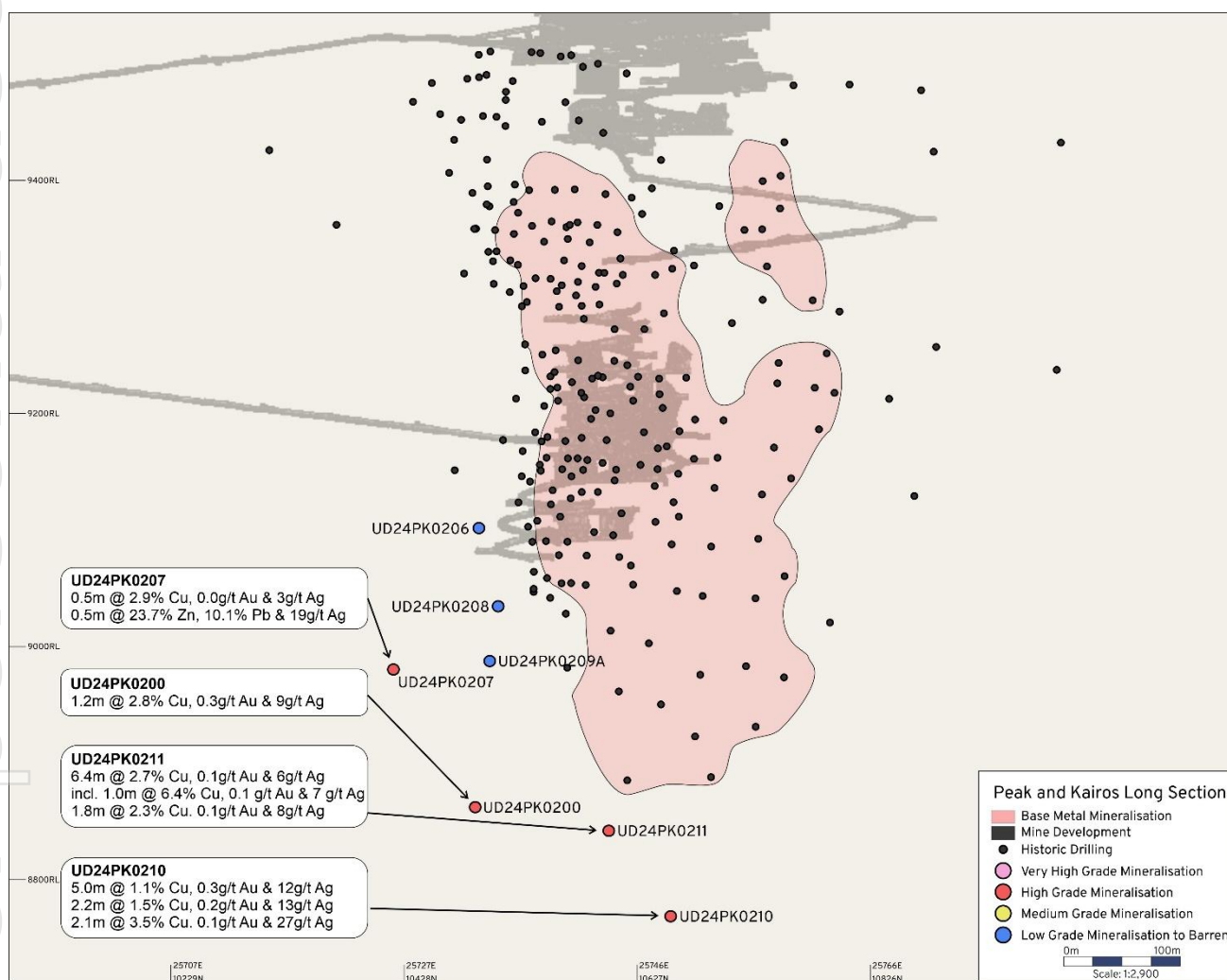
Figure 4: Long section of the Kairos and Peak deposits showing mine development, visible mineralisation envelopes, existing drilling and currently reported drillholes.
