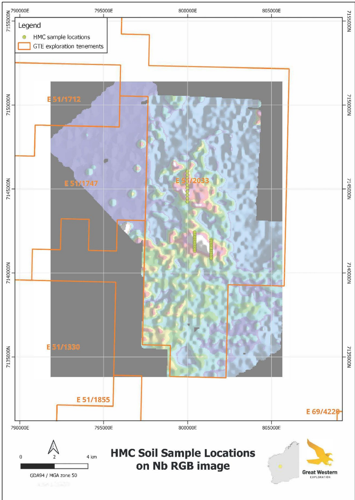
Figure 7: Locations of the heavy mineral concentrate samples taken at Sumo. Background image is the niobium Z-score lag-soil anomalism at Sumo (GTE ASX Announcement 16 October 2024).
