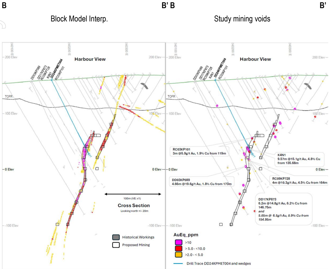
Figure 7: DD24KPMET004 in cross section. Gold equivalent results displayed filtered for intervals >2.0g/t AuEq. The plan location and orientation of the cross section is provided in Annexure 1.
