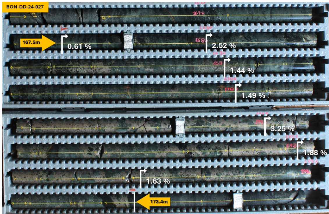
Figure 7 – Nelore Prospect – core photo from drill-hole BON-DD-24-027 Stringer and semi-massive sulphides → pyrrhotite (brown-bronze colour) > chalcopyrite (brassy yellow) > pyrite. Assays returned 5.9m @1.93% Cu from 167.5m.
