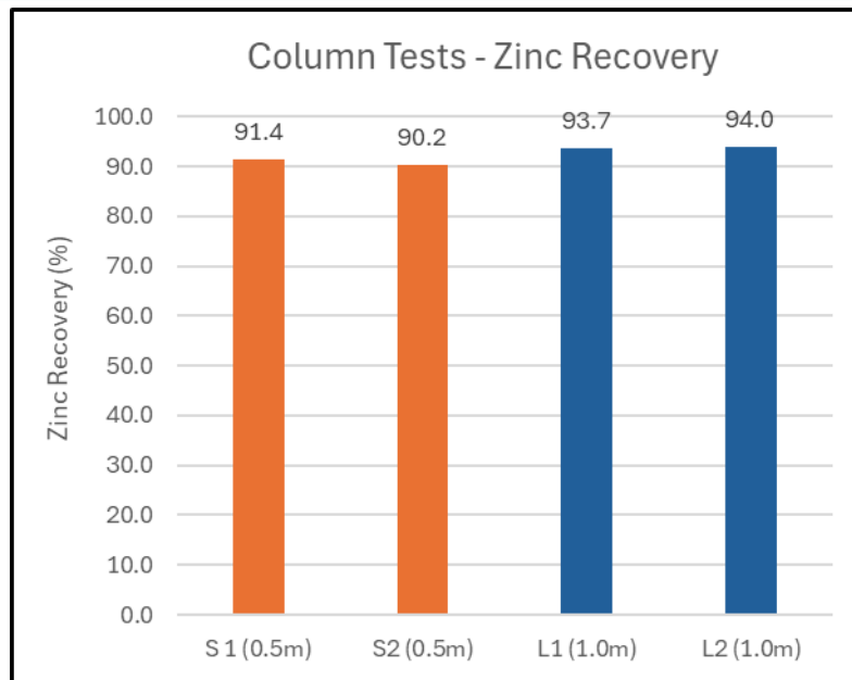
Figure 3: Zinc recovery achieved in 0.5m 8 and 1.0m column tests
