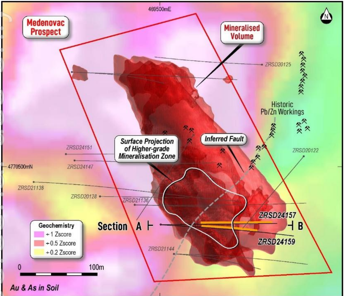
Figure 5. Plan view map of the Medenovac Prospect, showing the surface projection of the higher-grade mineralisation zone, the broader drill-defined mineralised (>0.5g/t AuEq) volume, drill traces, historical workings and background gold + arsenic in soil geochemical response.
