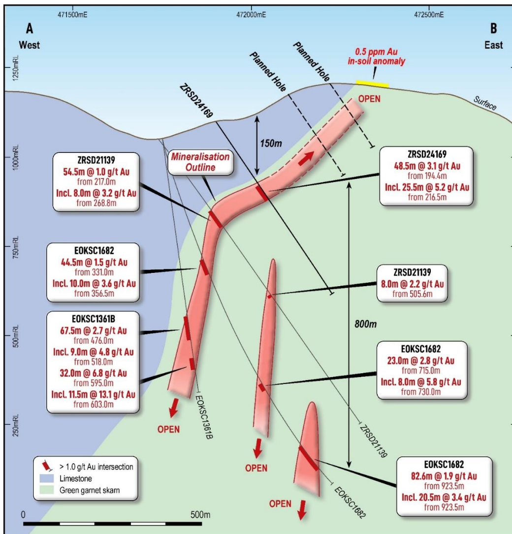
Figure 8. Gradina cross-section, showing results for ZRSD24169 and historical drilling with background geology.
