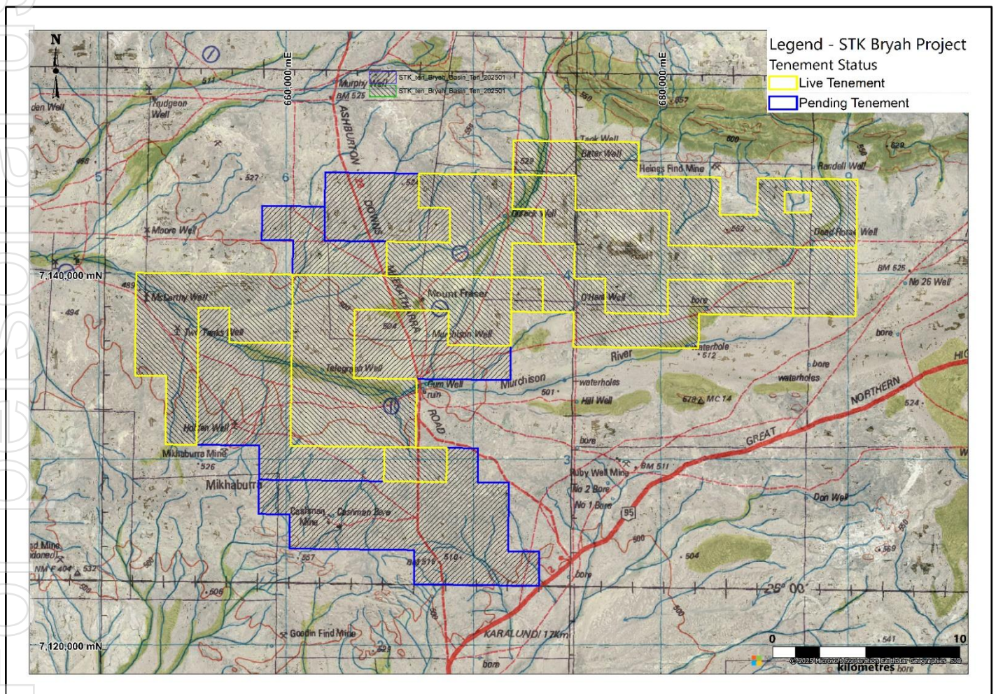
Figure 18. Bryah Basin tenement portfolio, highlighting both the live and pending tenement applications in relation to 250K topo underlay image.
