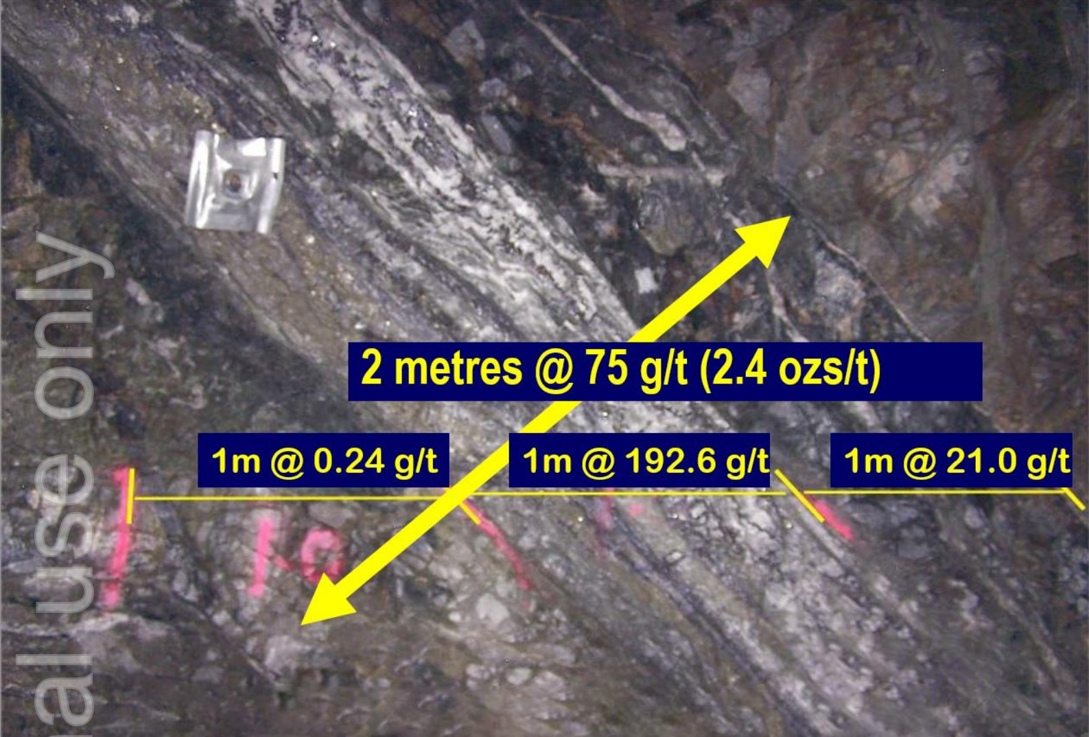
Underground image from previous test mining at Charters Towers, showing a gold-bearing reef with mineralisation including 2 metres at 75 g/t (2.4 ozs/t) and additional intervals of 1 metre at 192.6 g/t and 1 metre at 21.0 g/t. The image highlights a quartz vein hosting gold together with lead and zinc sulphide (galena and sphalerite) mineralisation. Lead and zinc sulphides are common geological indicators of gold-bearing systems in the area. Source: See ASX Announcements: Quarterly Activities Report and Appendix 5B, dated 11 January 2022 and Mineral Resources and Ore Reserves 2020, dated 9 December 2020.
