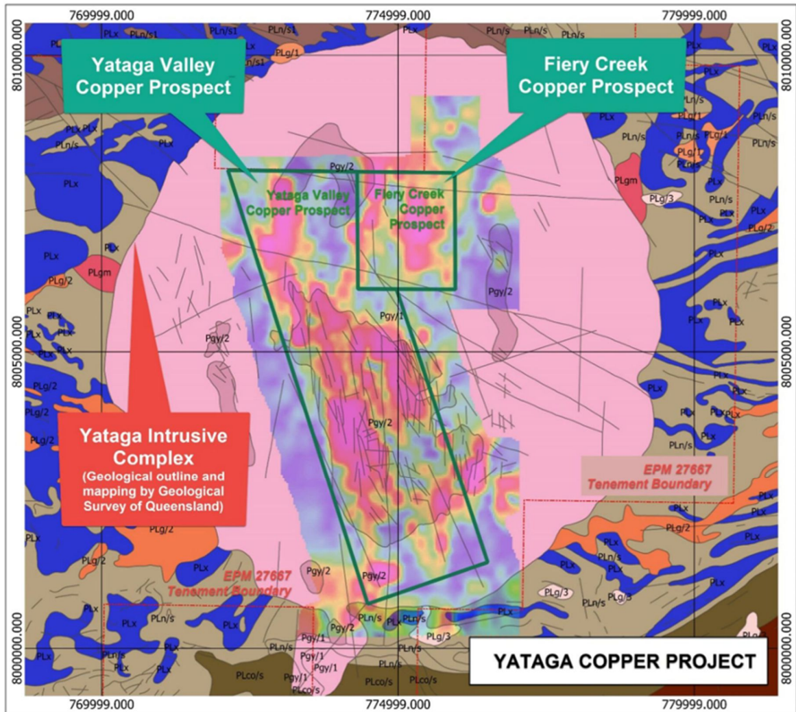
Figure 2. The Yataga Copper Project showing the locations of the two prospects – Fieri Creek Prospect and Yataga Valley Prospect overlaying the copper geochemistry anomalous zones (magenta) within the Yataga Igneous Complex
