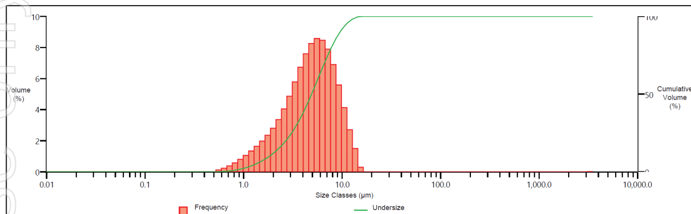
Figure 3: Particle Size Distribution (PSD) of the fines feed
