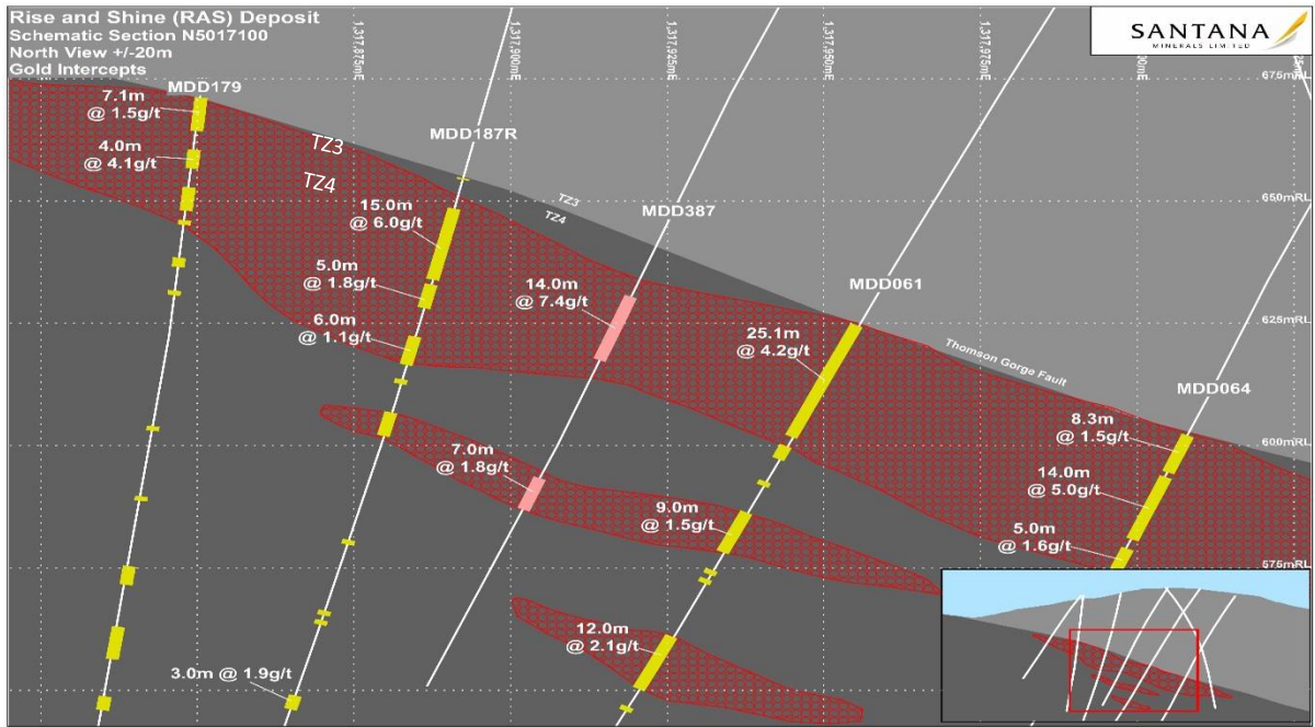
Figure 2. N5017100 section showing MDD387 and the correlation with the high-grade zones.
