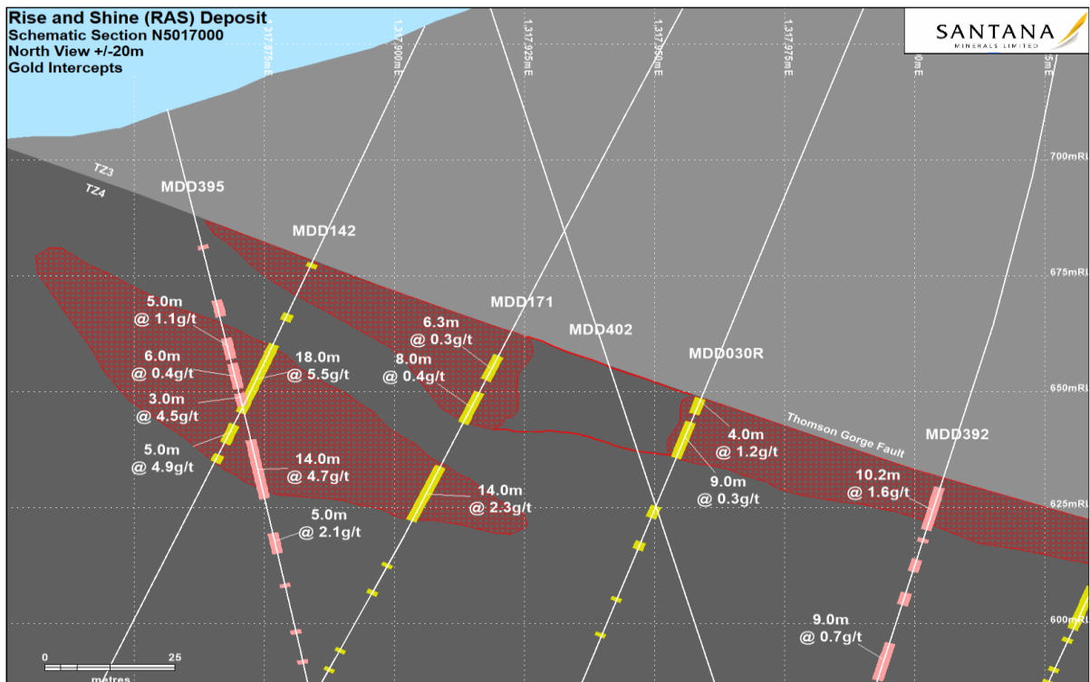
Figure 3. N5017000 section showing new intercepts of MDD395 and a planned target hole (MDD402).
