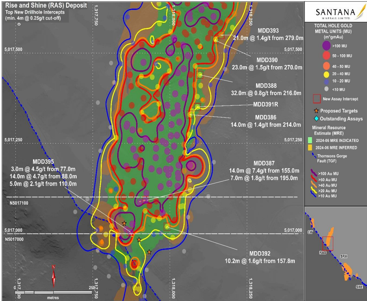
Figure 1. Plan of RAS metal unit (or gram.metre) map with pierce points of new drilling.
