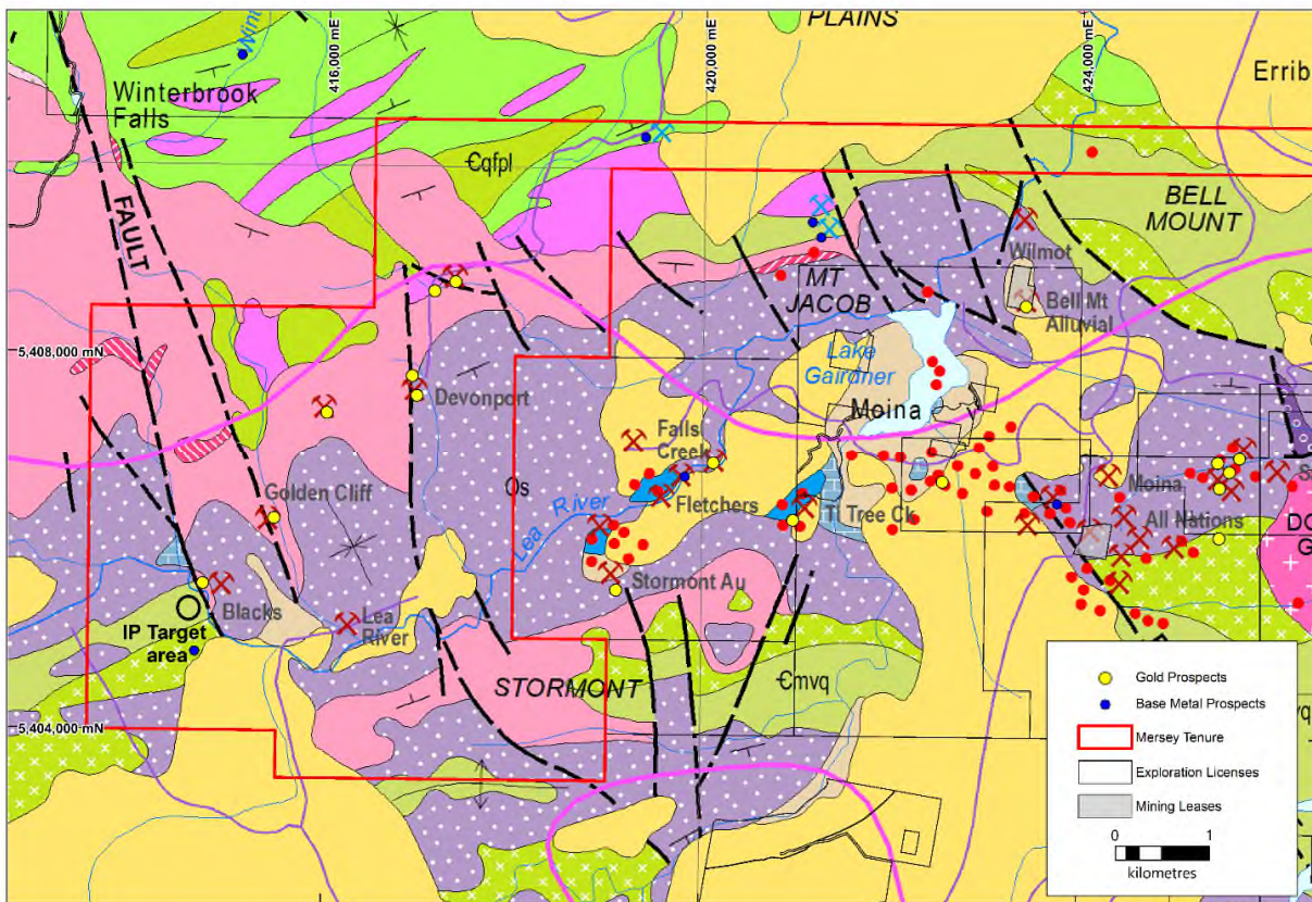
Figure 4. Geological Survey of Tasmania regional geological map of the Mersey Project area western tenure, showing key gold prospects identified in the MTR database. Also note, IP target areas to further investigate (Coords GDA 94 MGA Zone 55)
