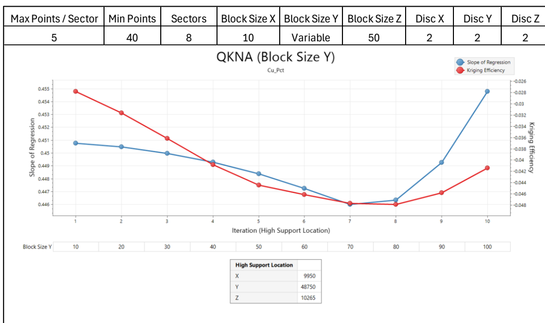
Figure 5-14: Block Size Parameter Direction Y Optimisation
