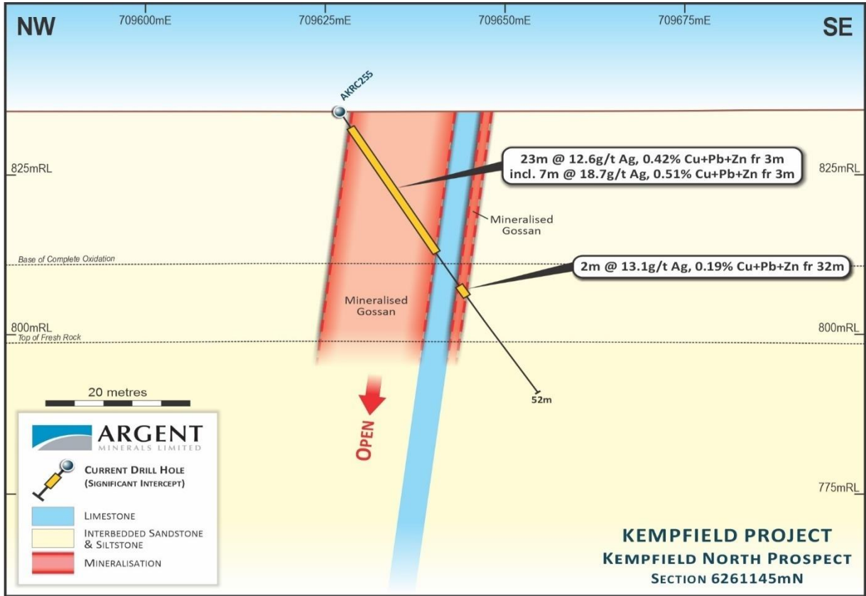
Figure 3 – Kempfield NW Cross Section 6261145N highlighting mineralised intervals
