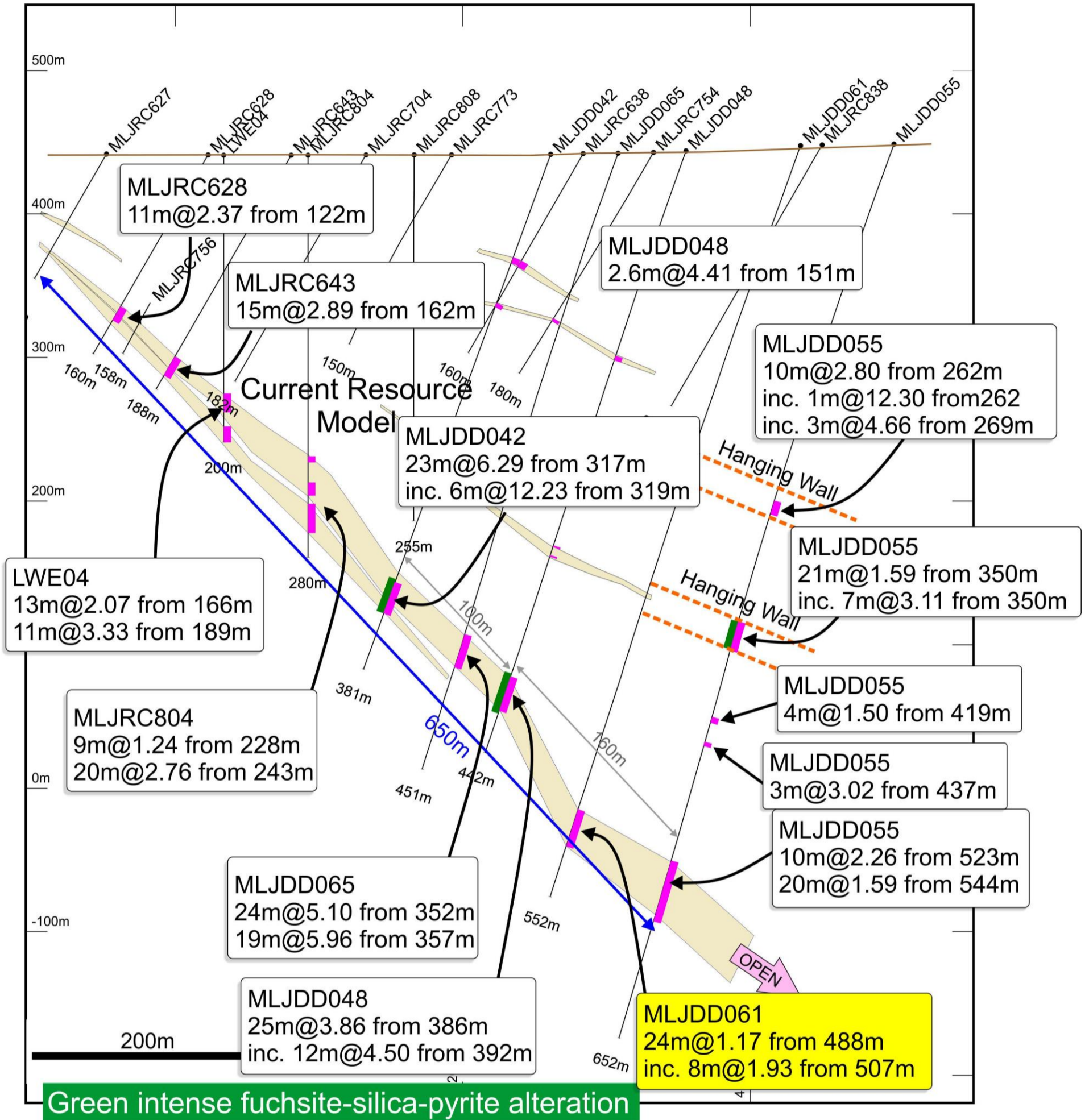
Figure 3. Cross section for LNJ4 northern area showing high-grade dipping gold zone containing resource model outline and MLJDD042, 48, 55, 65 and 61 being part of a large 650m down dip footwall down dip extension of 160m from MLJDD048.
