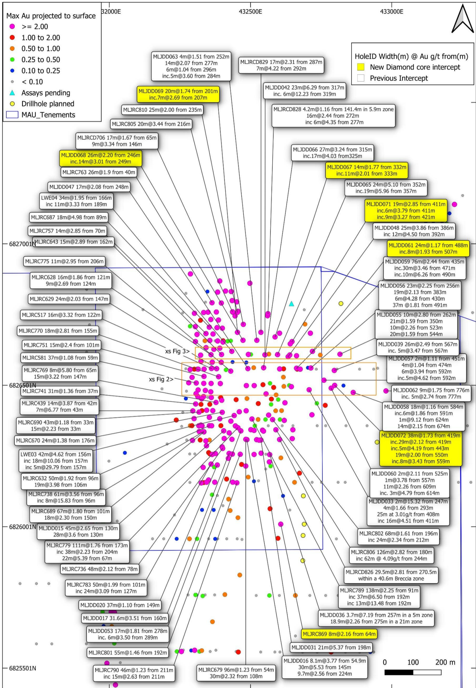
Figure 4. The Lady Julie North 4 deposit has numerous significant thick intersections from the latest drill programme (yellow large rectangular label) and previous drilling (white label) with maximum gold projected to surface and planned deeper drillholes (in yellow).
