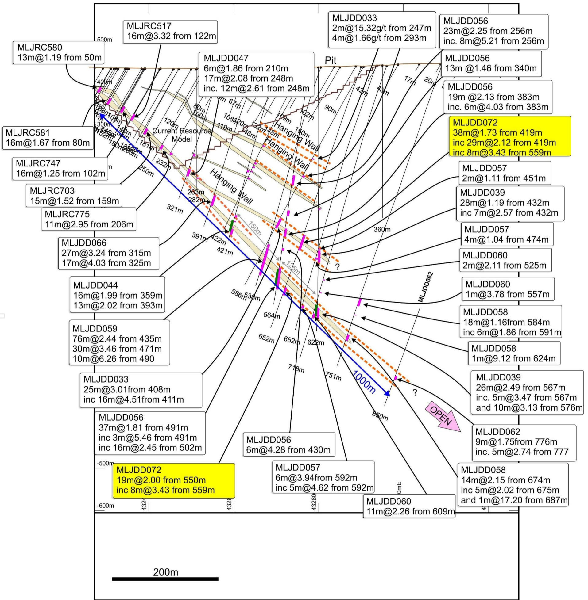
Figure 2. Composite section for LNJ4 central area showing high-grade dipping gold zone containing resource model outline, proposed open pit and MLJDD039, 44, 47, 56, 57, 58, 59, 60, 62, 66, 72 being part of a very large 1000m down dip mineralised main zone.
