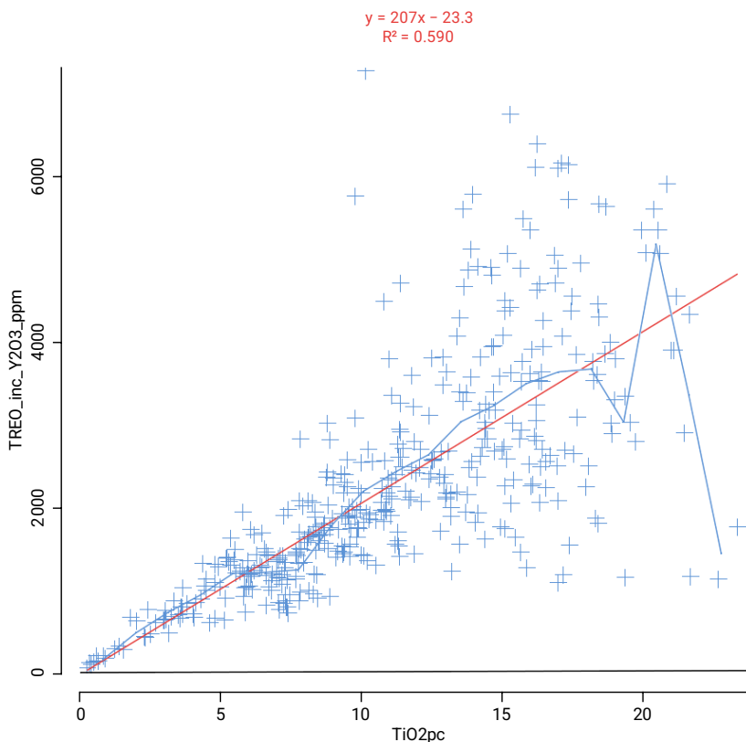
Scatter graph of TREO_inc_Y2O3_ppm vs TiO2pc
