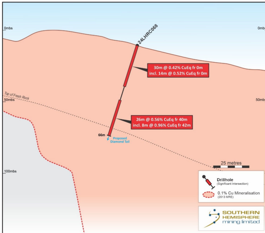
Figure 4. Cross Section showing RC 24LHRC068 which ended in mineralisation and ready for diamond drilling tail to depth.
