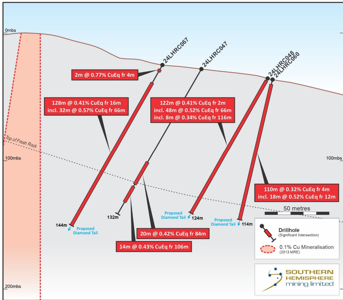
Figure 5. Cross Section showing RC 24LHRC067, 48 and 60 which all ended in mineralisation and ready for diamond drilling tail to depth in a new extension zone south.
