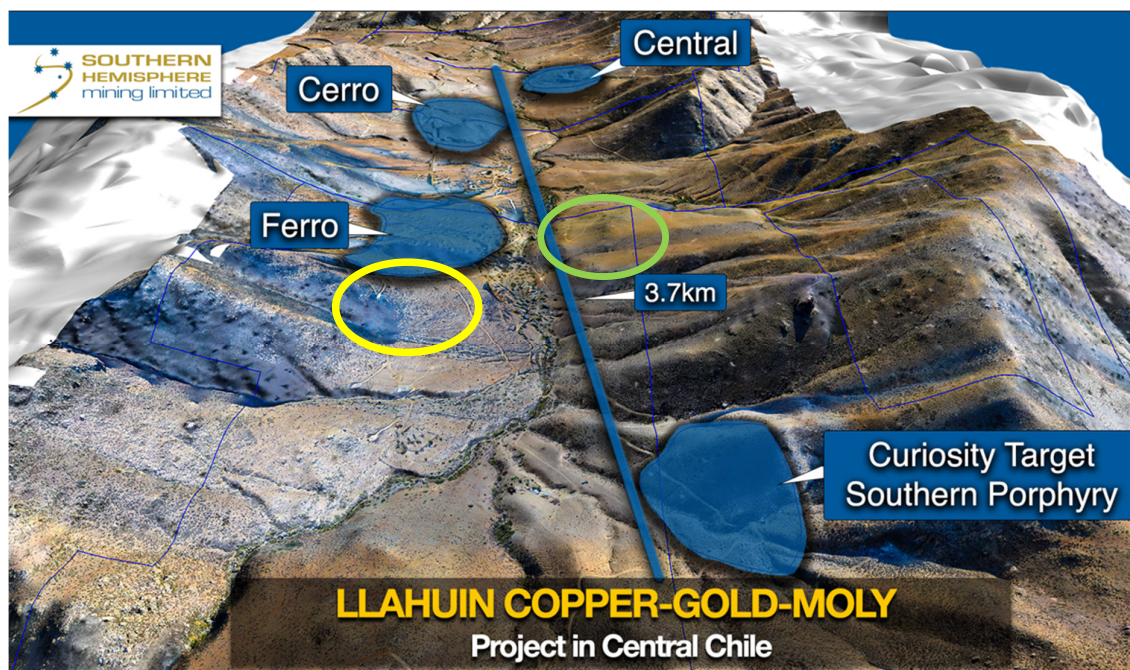
Figure 10. 3D view looking northeast from the Curiosity target - Southern Porphyry to Central Porphyry, showing the scale of the large Llahuin mineralising system with Ferro extension in yellow circle, and the newly identified East Porphyry zone in the green circle (colluvium covered up to 5m deep).
