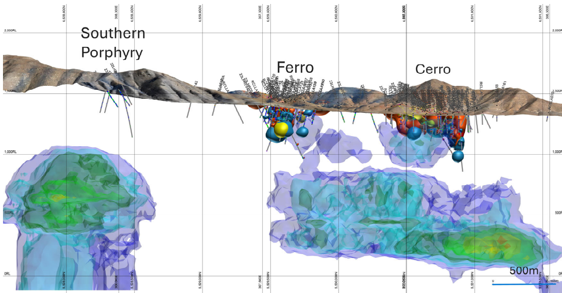
Figure 14. A similar long section to Figure 11, this time showing from Southern Porphyry (Curiosity Target at depth) to Cerro, showing similar spatial relationships.
