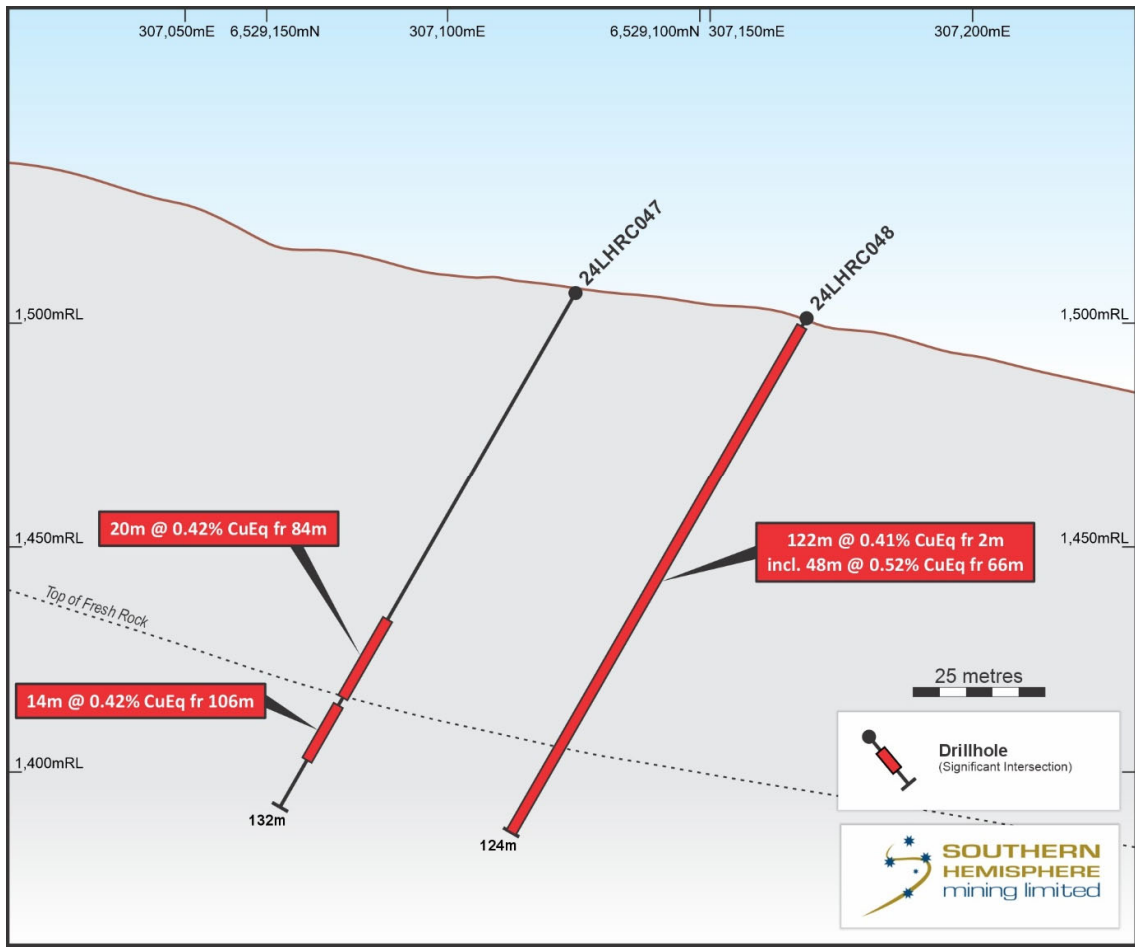
Figure 6. Cross section showing 24LHRC047 and 24LHRC048. This is a new area of mineralisation outside of the current Mineral Resource, potentially adding tonnage.
