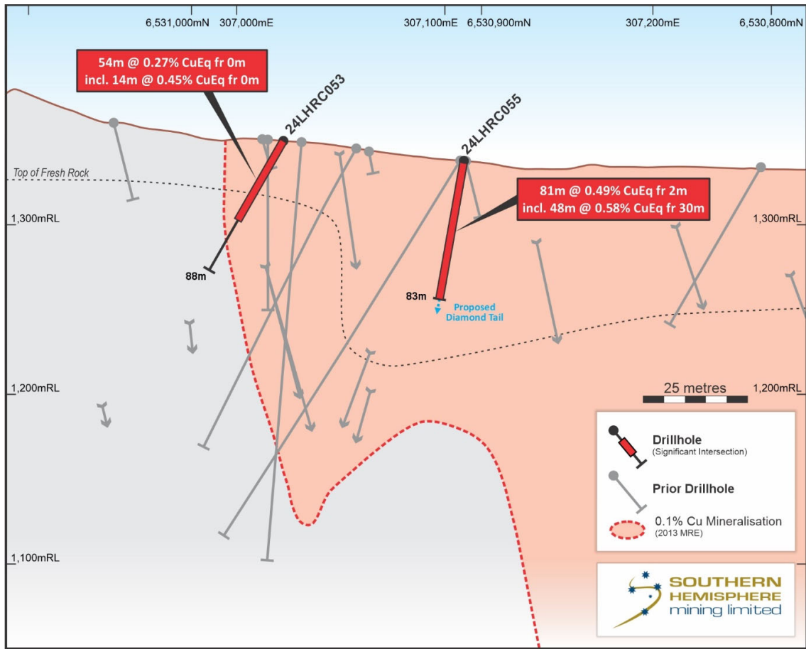
Figure 8. Cross section showing 24LHRC053 and 24LHRC055. 24LHRC055 will be extended with a diamond tail.
