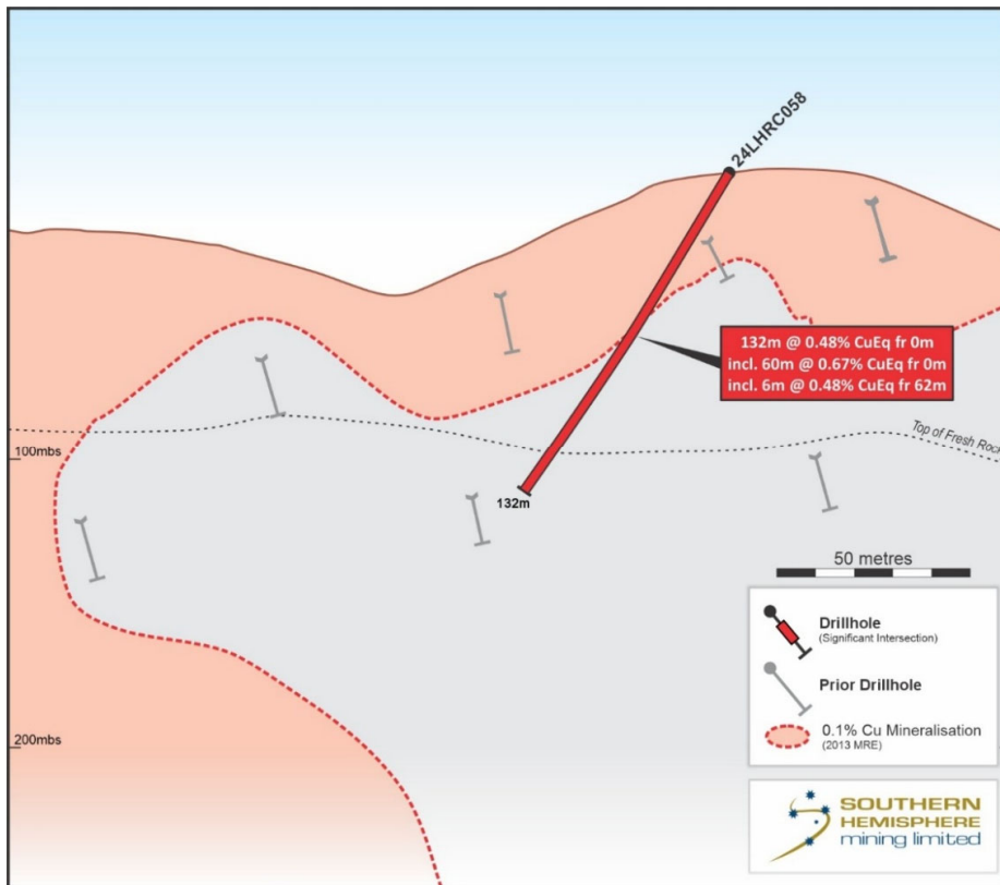
Figure 3. Cross section showing 24LHRC058, which will be extended by diamond drilling.
