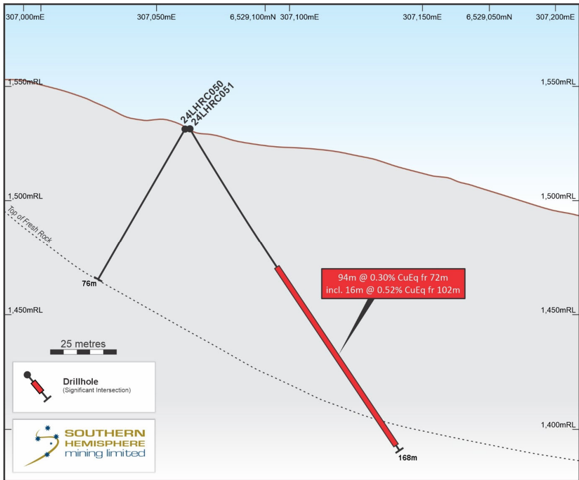
Figure 7. Cross section showing 24LHRC050 and 24LHRC051, and new mineralised zone outside of the current Mineral Resource.
