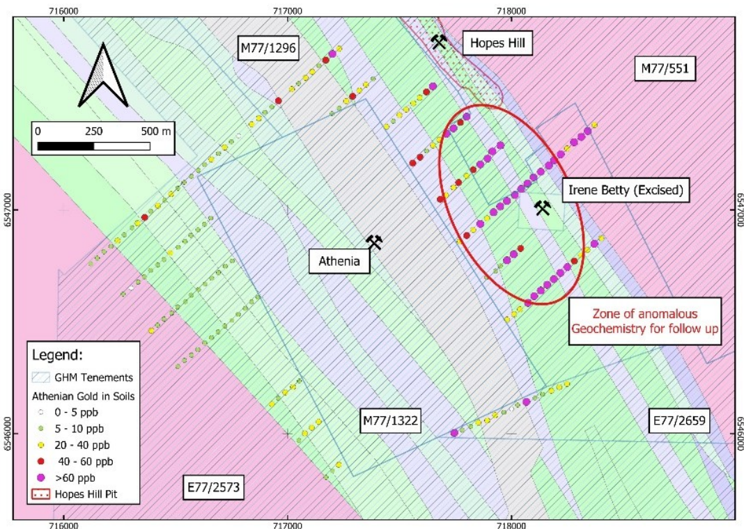
Figure 4: Athenia Soil Anomaly.
