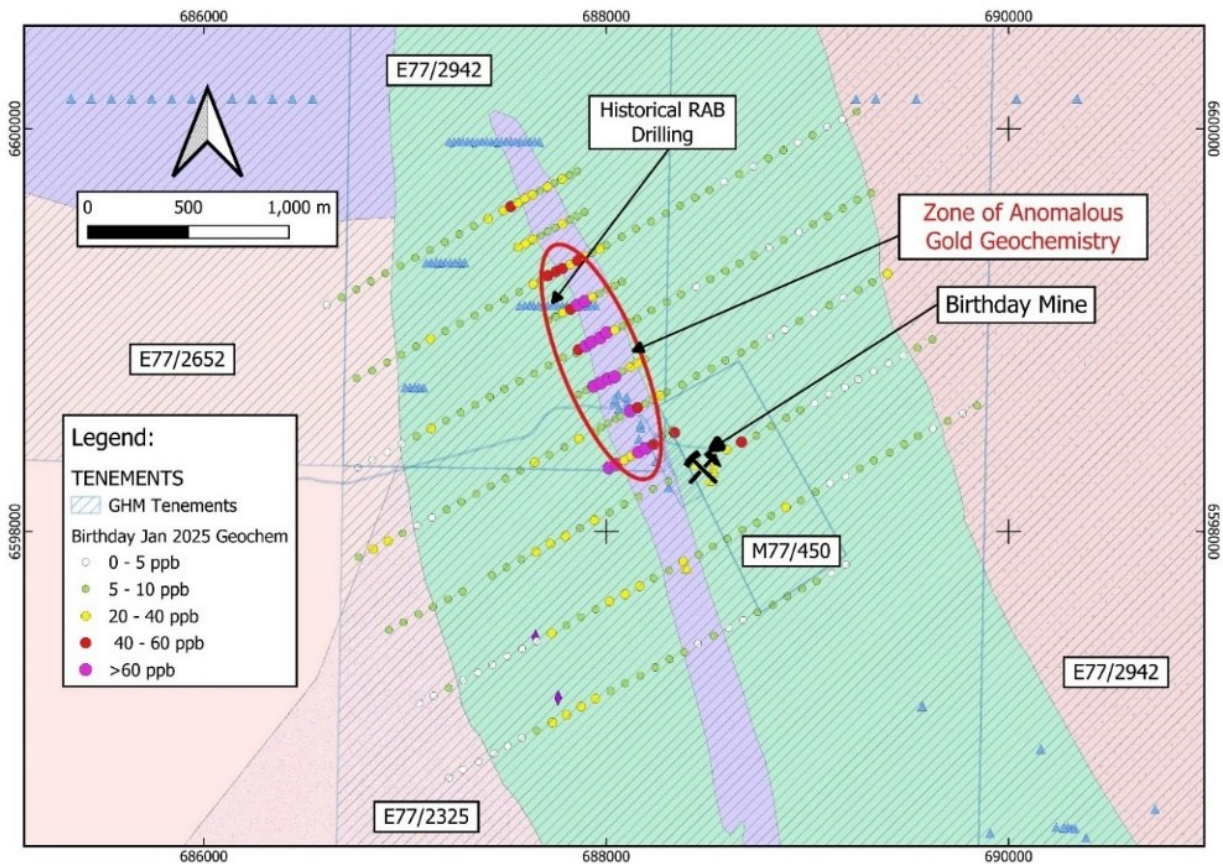
Figure 3: Birthday Soil Anomaly.
