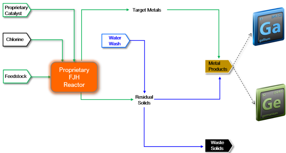
FIG. 4: conceptual flowsheet for testwork employed
