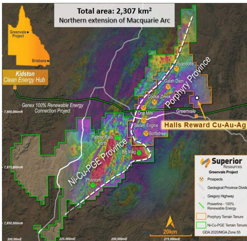
Figure 1. Greenvale Project regional magnetics with the location of the high-grade Halls Reward Cu-Au-Ag mine. Additional nearby high-grade Cu deposits include Wyandotte and One Mile, alongside the Company's large-scale porphyry Cu-Au discoveries at Bottletree and Cockie Creek.
