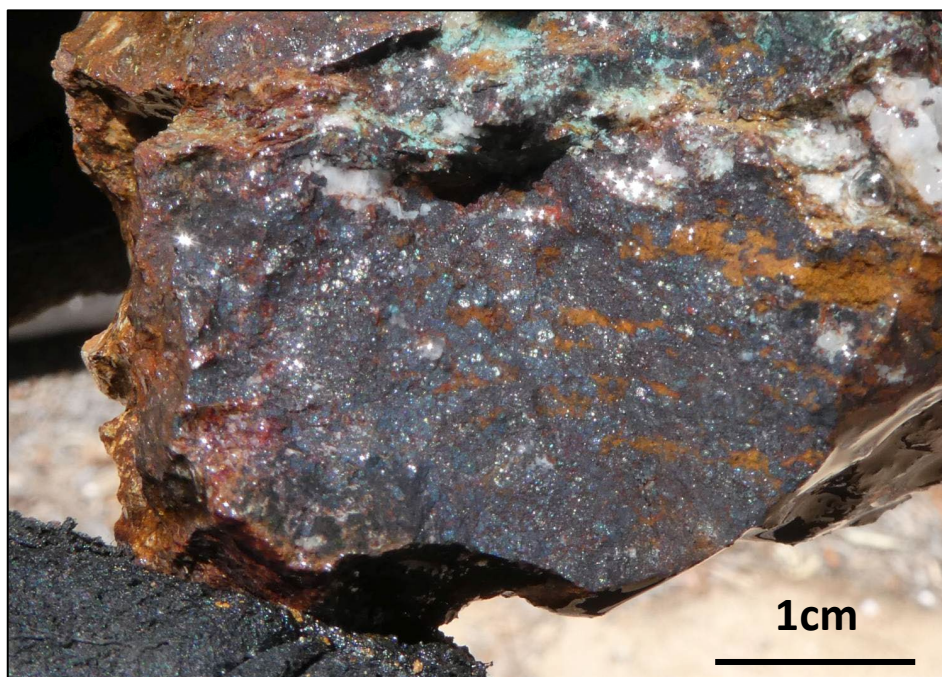
Figure 7. Main Lode chalcocite with remnants of chalcopyrite and malachite; not assayed.
