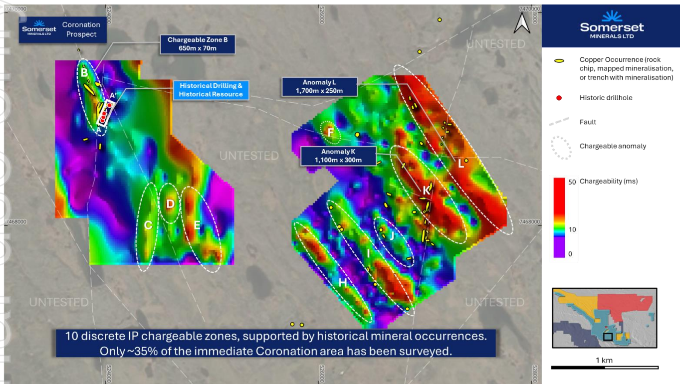
Figure 1: Reprocessed IP survey showing chargeable zones at Coronation Prospect, coincident mineral observations, and highly anomalous drill targets K and L.
