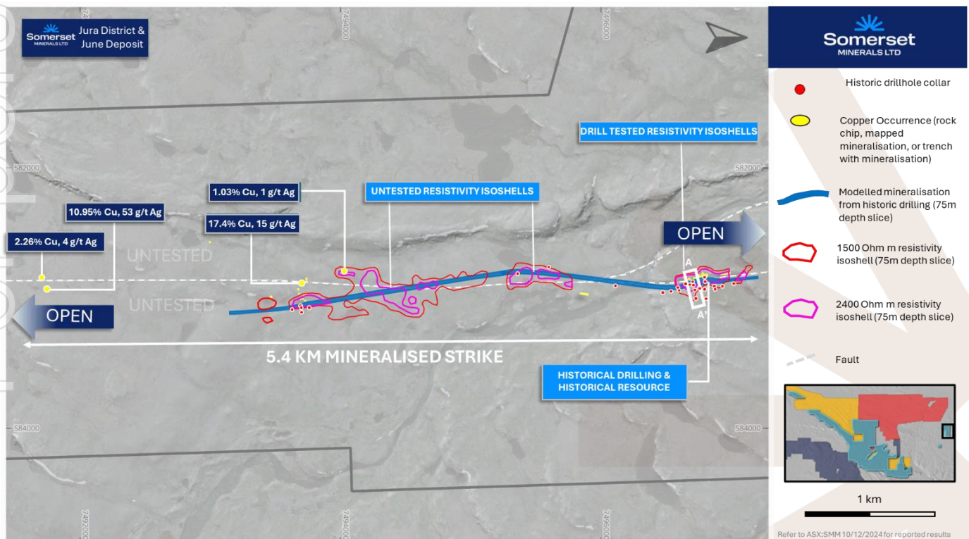
Figure 2: Reprocessed resistivity survey showing resistivity isoshells within the Jura District, and coincident mineral observations
