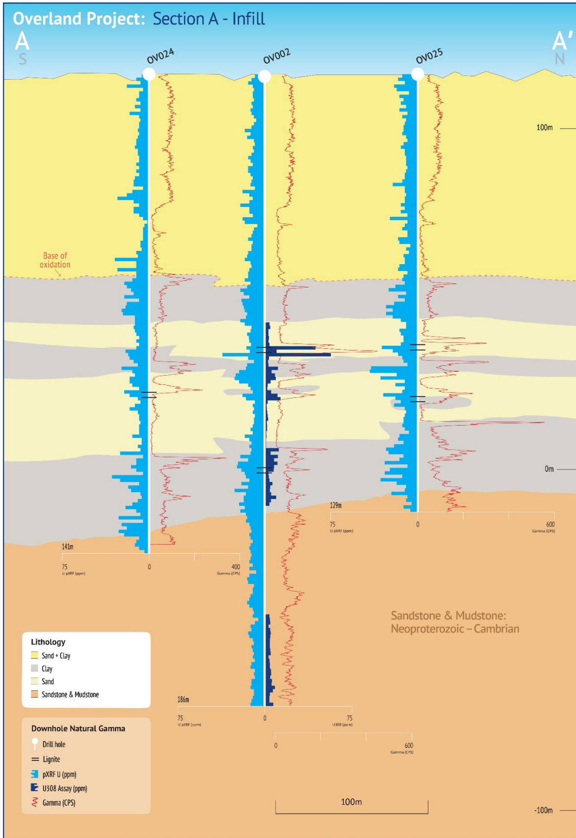
Figure 4: Section showing OV002. OV002 intersected 1m @ 58ppm U 3 O 8 from 82m. Assay results from OV024 and OV025 are pending
