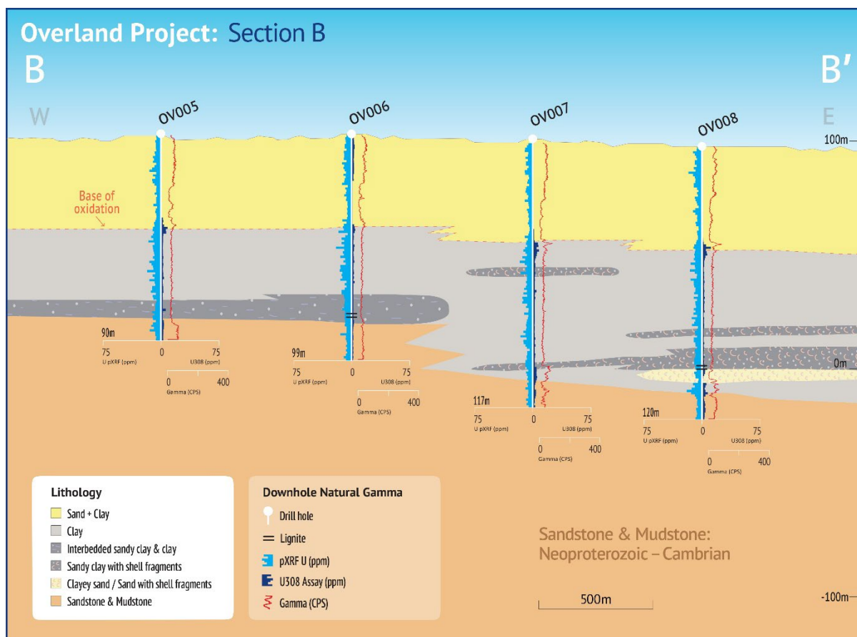
Figure 5 : Section B-B 1
