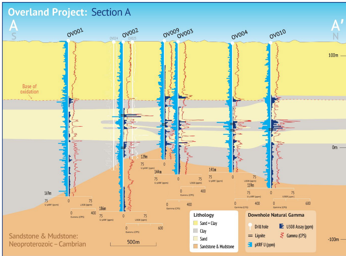
Figure 3: -Section A-A 1 See Figure 4 for OV002 detail
