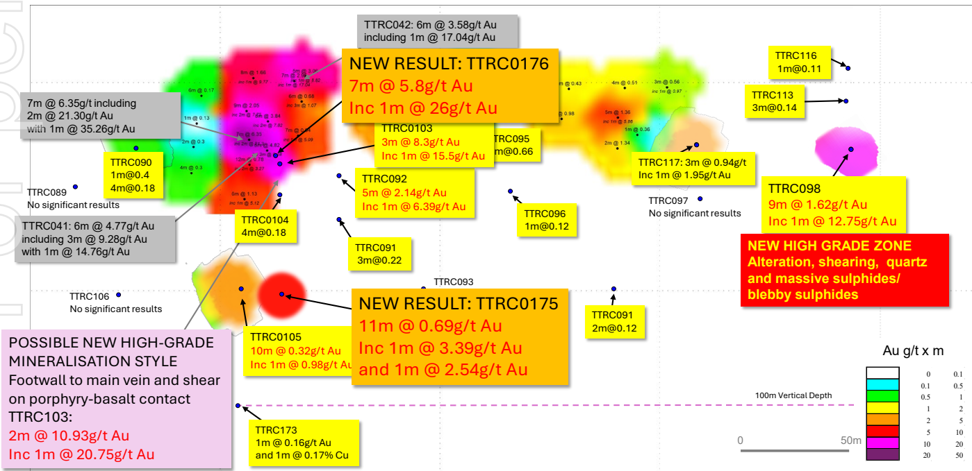
Figure 2: Long projection of the Central Main Kurundi mineralized zone beneath the central workings area. View is perpendicular to the main vein which dips approximately 35° towards 215°. New results shown in orange boxes, 2022 results shown in grey boxes, light purple box is for the footwall intersection.
