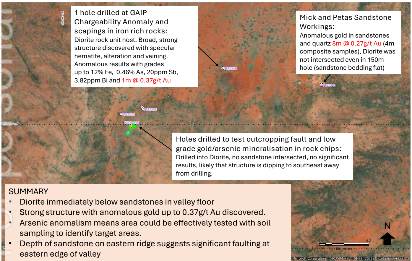
Figure 7: Tarragans North drilling and results summary.
