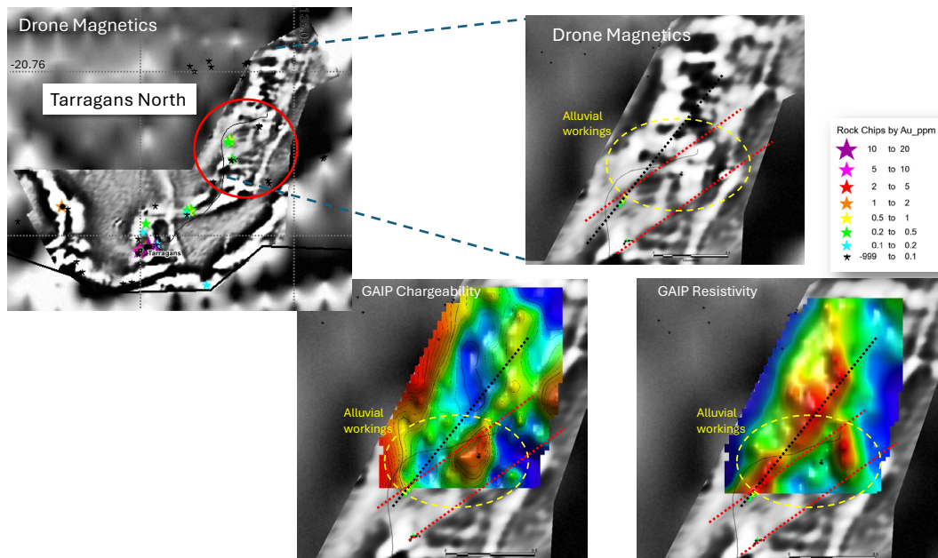
Figure 6: Tarragans North 2023 GAIP and Drone Magnetic Geophysical results.
