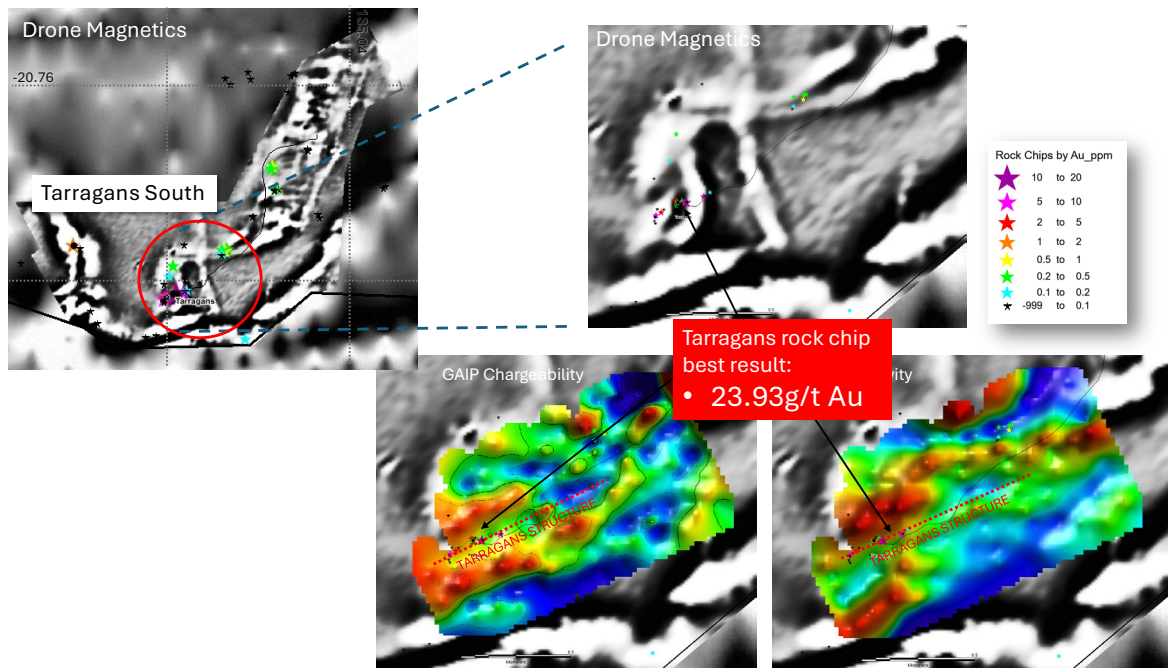
Figure 5: Tarragans South 2023 GAIP and Drone Magnetic Geophysical results.
