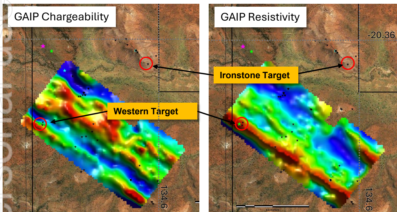
Figure 9 Millers GAIP results: left Chargeability, right Resistivity.
