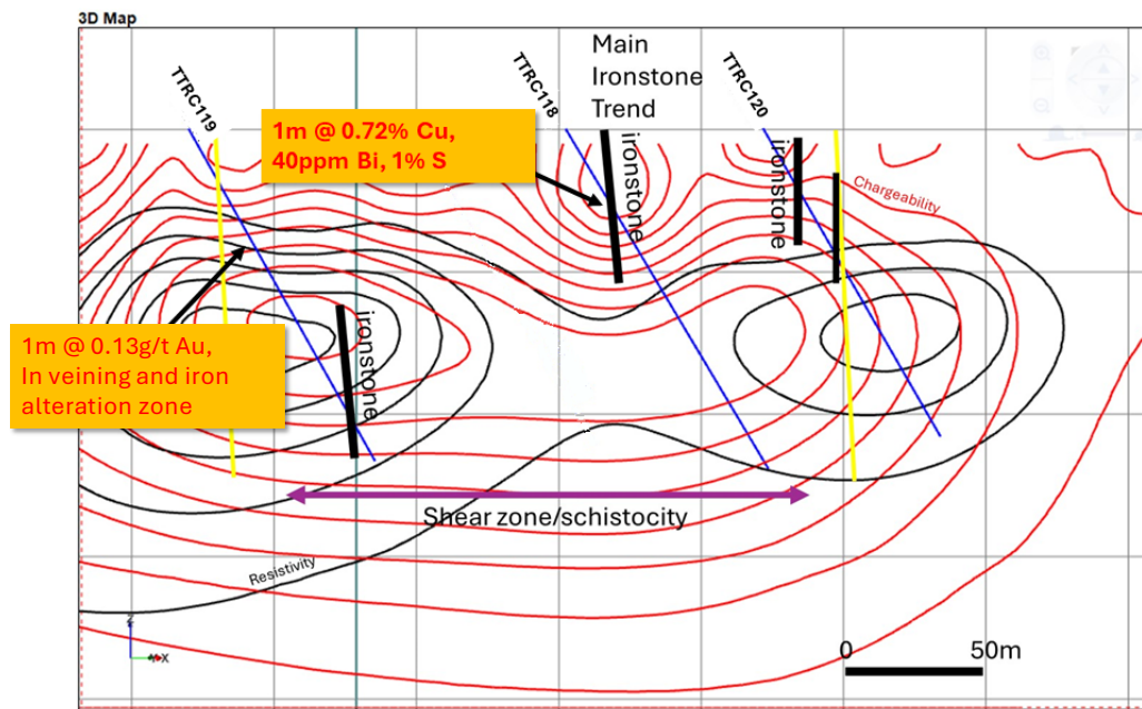
Figure 10: 3D oblique section (facing NW) of Millers DDIP Resistivity (black lines) overlain by DDIP chargeability contours (red lines) and drilled RC holes (blue lines).
