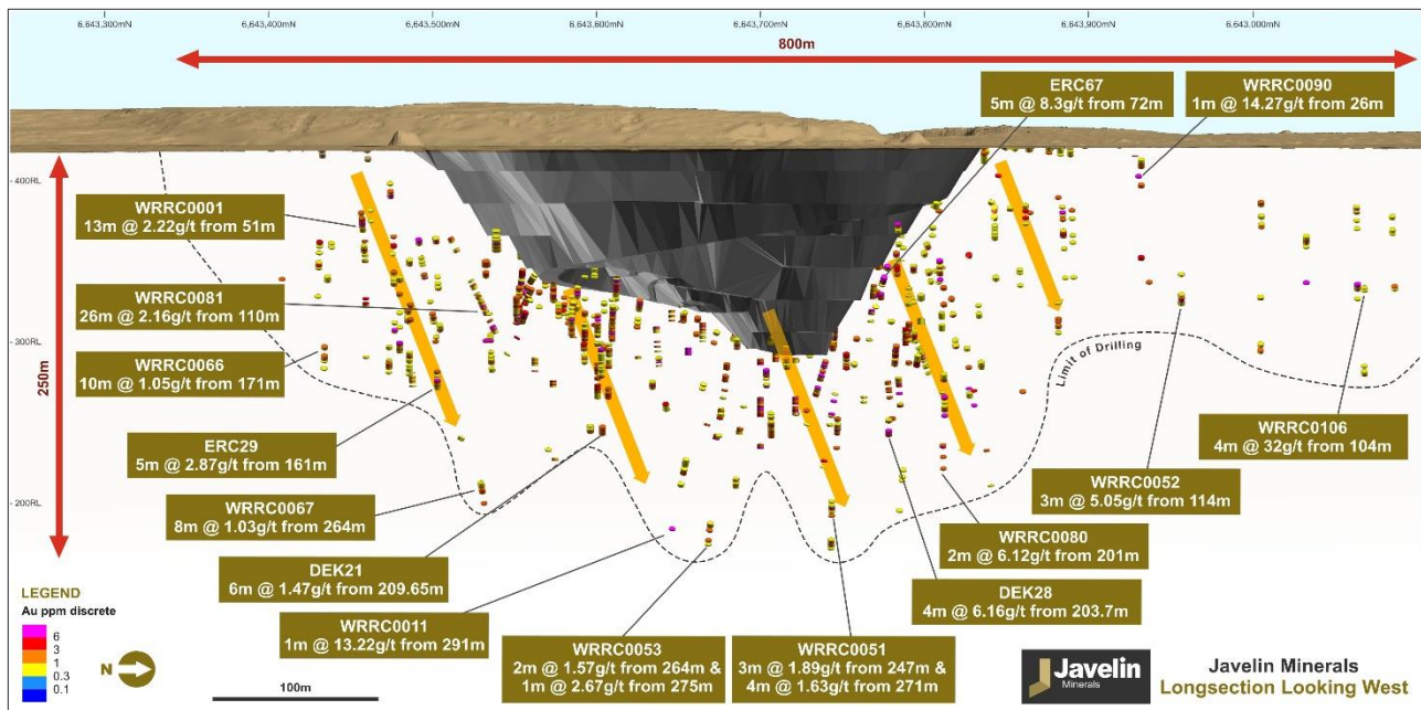
Figure 4 – Long Section showing significant gold intersection along with the main mineralised projected gold lodes looking west of the Eureka Pit
