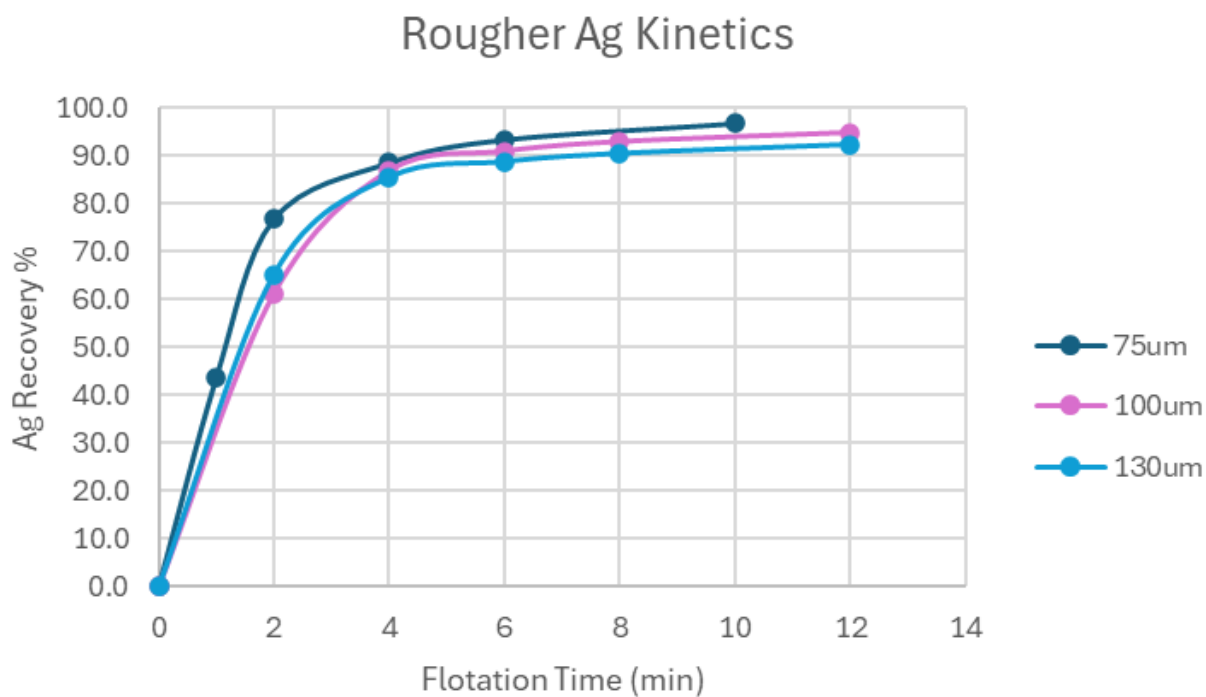
Figure 3: Maronan Carbonate-hosted silver-lead ore, rougher silver recovery with time for a range of grind size factions.
