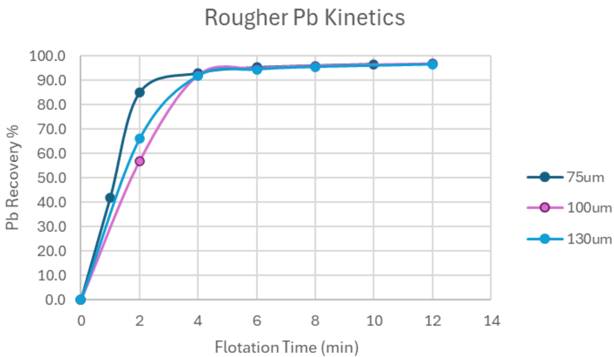
Figure 2: Maronan Carbonate-hosted silver-lead ore, rougher lead recovery with time for a range of grind size factions.
