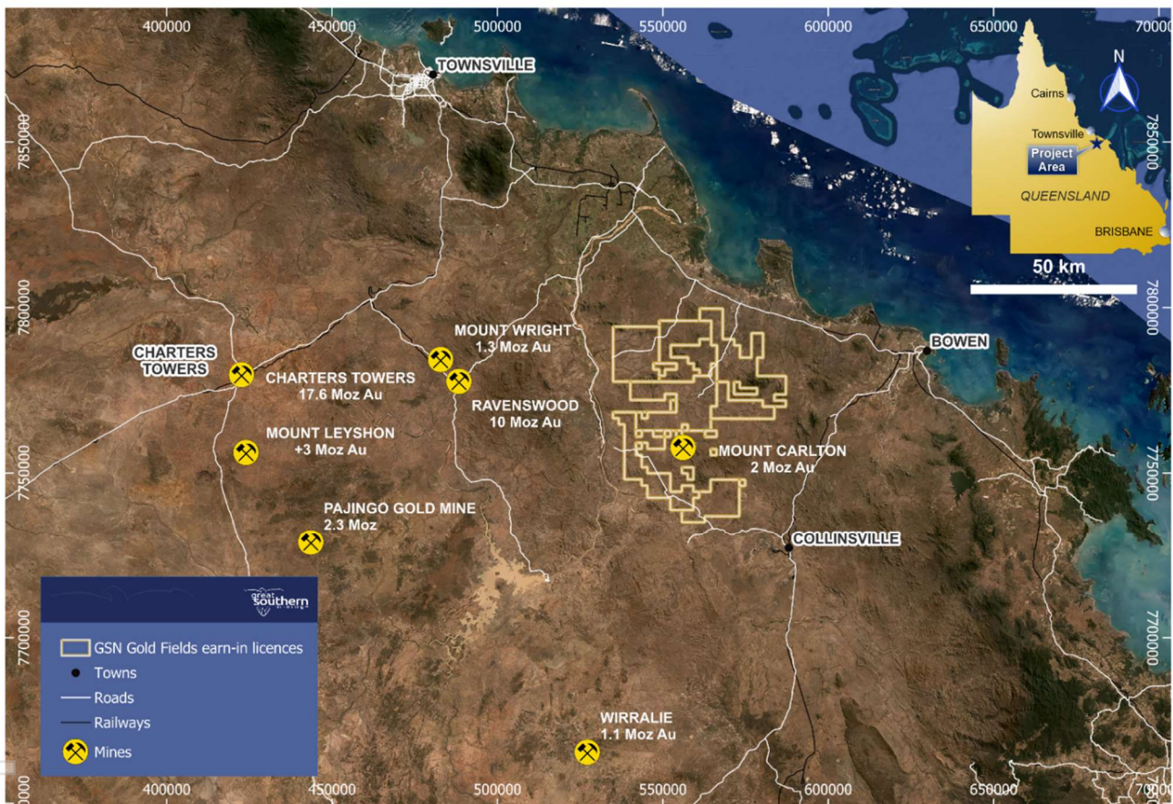
Figure 6. Location map showing major intrusive related gold systems (IRGS) and their gold endowment proximal to Edinburgh Park.
