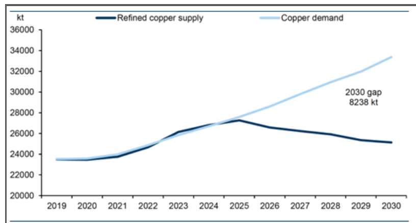
Figure 7 - Copper Supply Gap Projection 4
