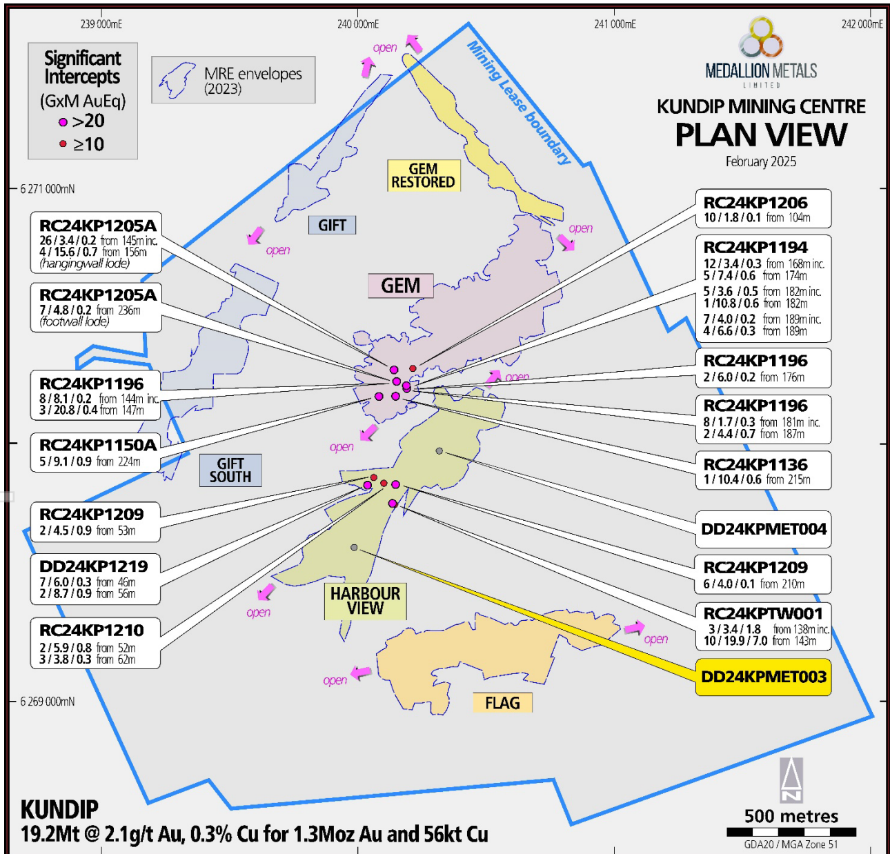
Figure 2: Plan view of KMC showing 2024-25 reported drilling results above 10 GxM AuEq and the location of DD24KPMET003 (Yellow Hole ID).
