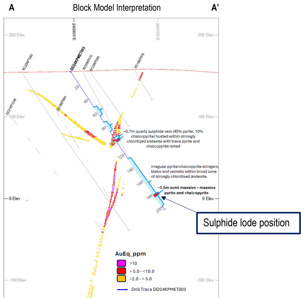
Figure 3: DD24KPMET003 in cross section. The plan location and orientation of the cross section is provided in Annexure 1.
