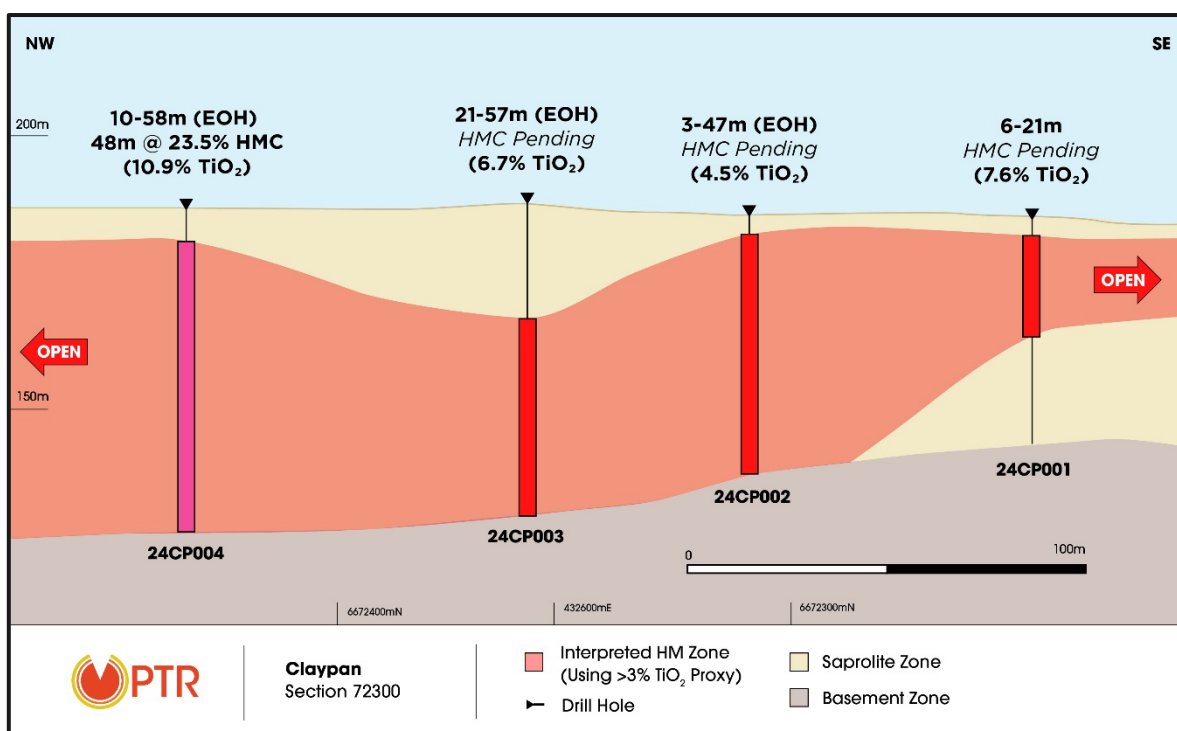
Figure 6: Claypan Prospect – Cross section 72300 showing HM intercepts and extent of \text{TiO}_2 mineralisation.
