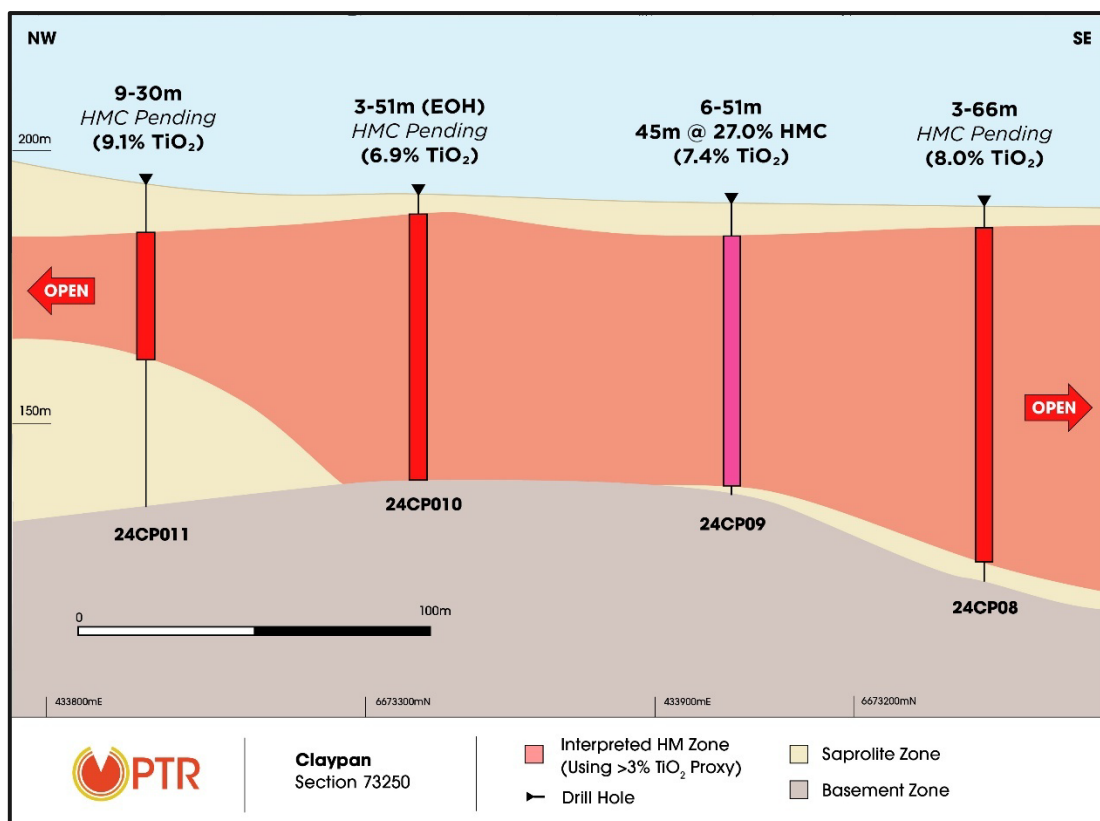
Figure 5: Claypan Prospect – Cross section 73250 showing HM intercepts and extent of \text{TiO}_2 mineralisation.
