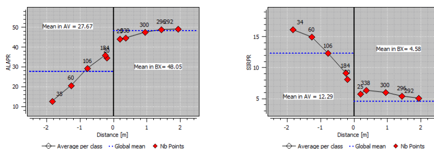
Figure 35 Contact analysis of the bauxite footwall, regarding the grades of Al_2O_3 and SiO_2 respectively, from Teófilo plateau
