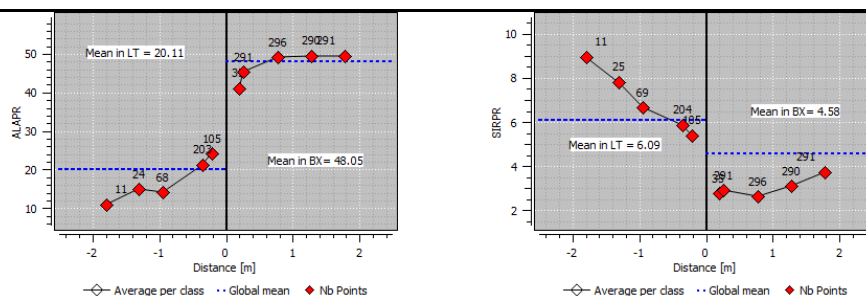
Figure 34 Contact analysis of the bauxite hangingwall, regarding the grades of Al_2O_3 and SiO_2 respectively, from Teófilo plateau
