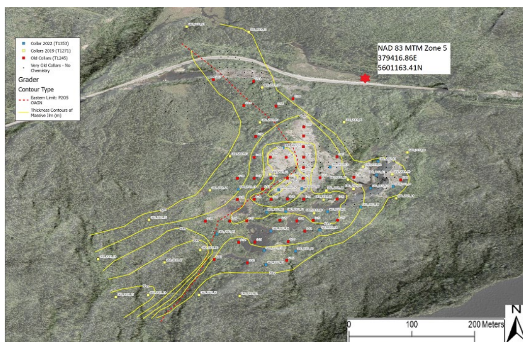
Figure 16 Plan view of the Grader deposit displaying the drill hole collar and elevation/thickness contours of the massive ilmenite domain. Starting east, the basal contact of the massive ilmenite domain with an above sea level (ASL) altitude of 180 m dipping southwest to a 50 m ASL. Yellow lines represent 20 m isopach contours
