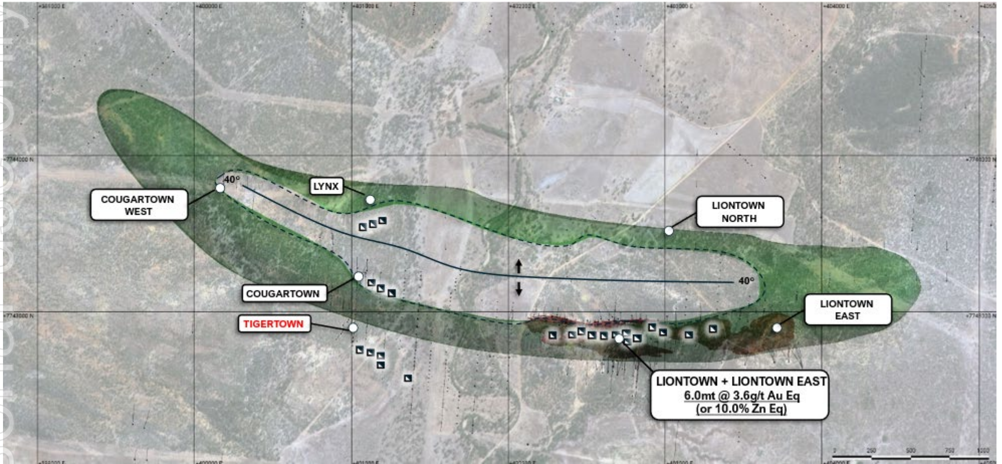
Figure 5: Plan view of the Liontown Dome (green surface) showing Tigertown location and historic workings (black/white squares).
