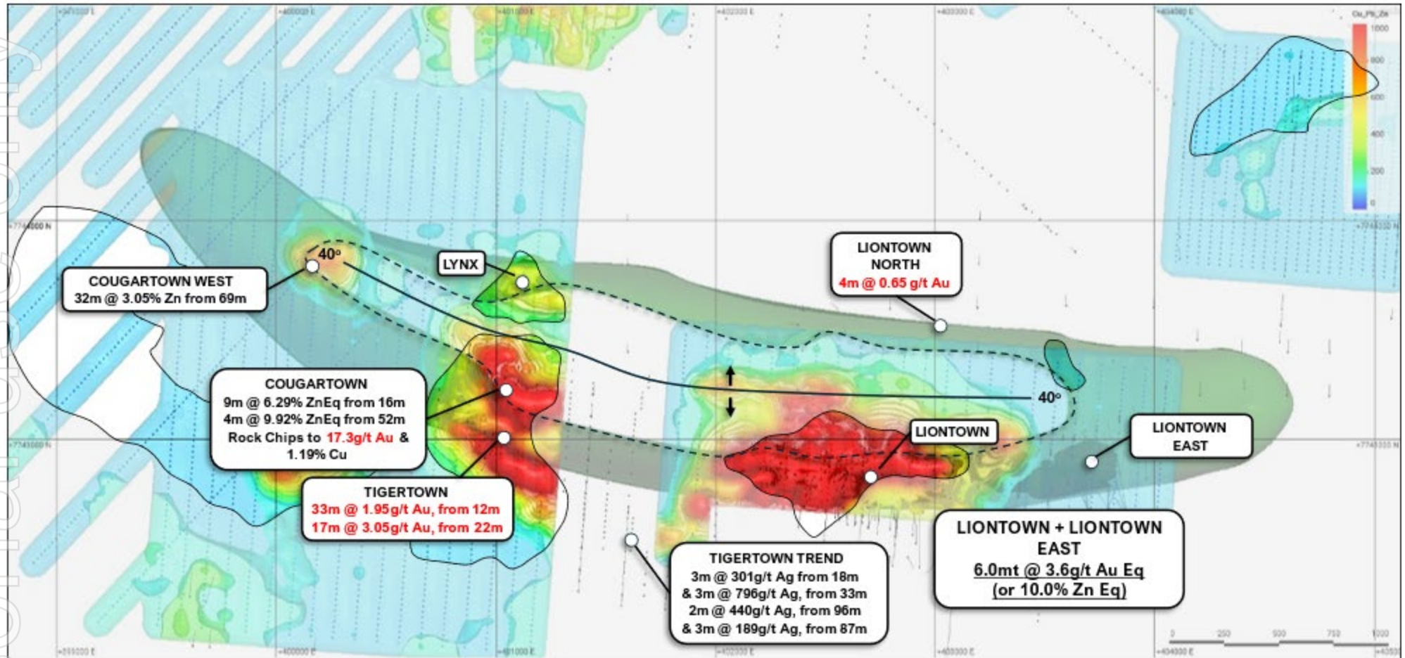
Figure 6: Plan view of the Liofntown Dome, showing contoured soil anomalism (Cu+Zn+Pb in soils) with key prospects and historic drilling results annotated. Areas of outcrop or subcrop (effective soil sampling) are highlighted within the black outlined shapes.
