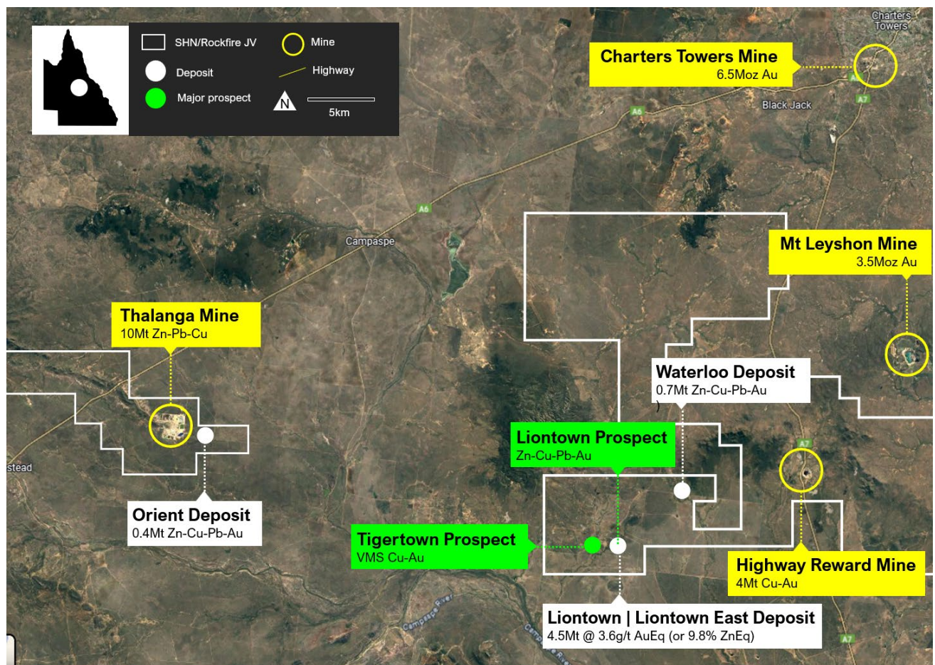
Figure 3: Tigertown is located approximately 1.2 km west of Liontown on the southern margin of the newly interpreted Liontown Dome.
